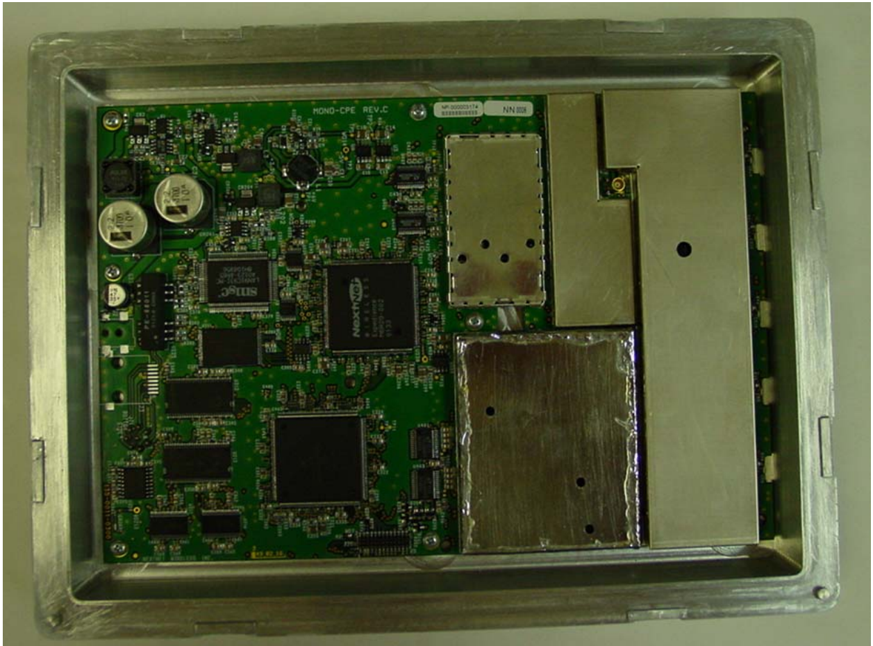
RF Board component side (with shields) in casting
