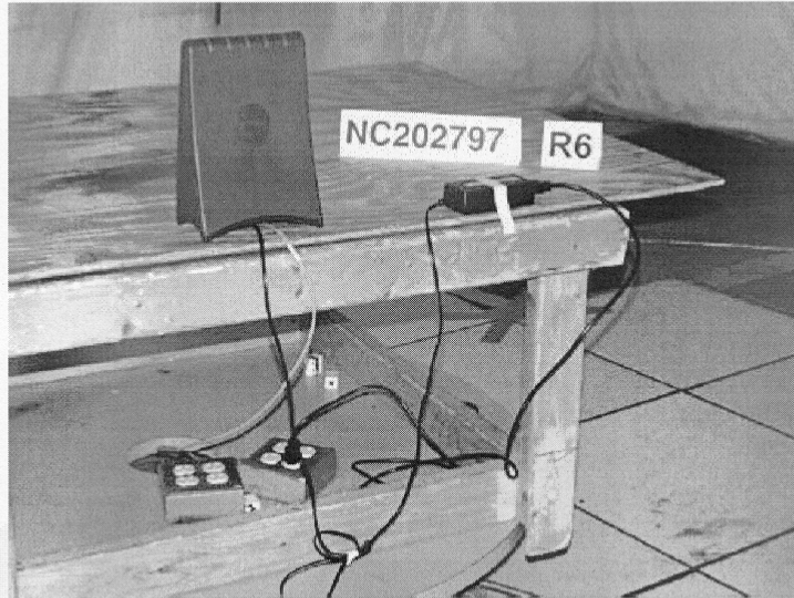
Test-setup photo(s): Radiated emission 30 MHz - 27000 MHz
