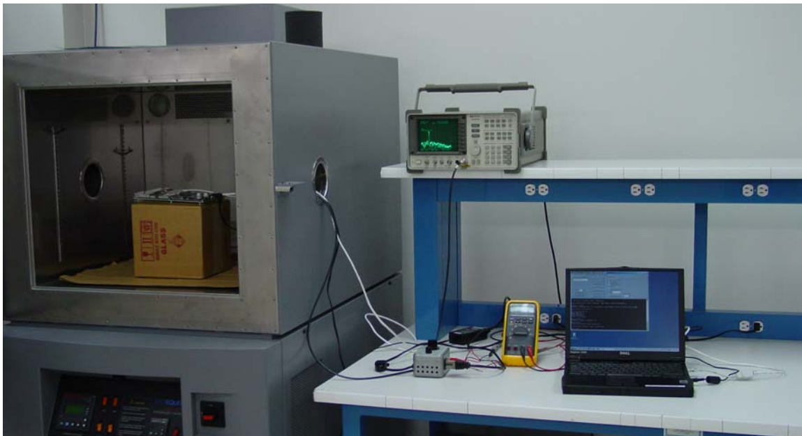
Frequency stability
