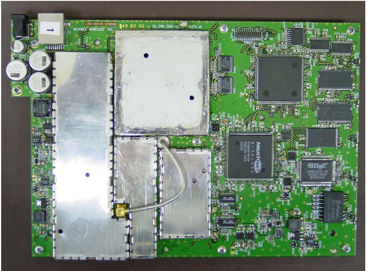
RF Board component side (with shields)
