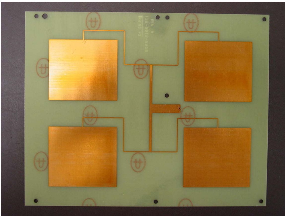
Horizontally Polarized Antenna (copper side)
