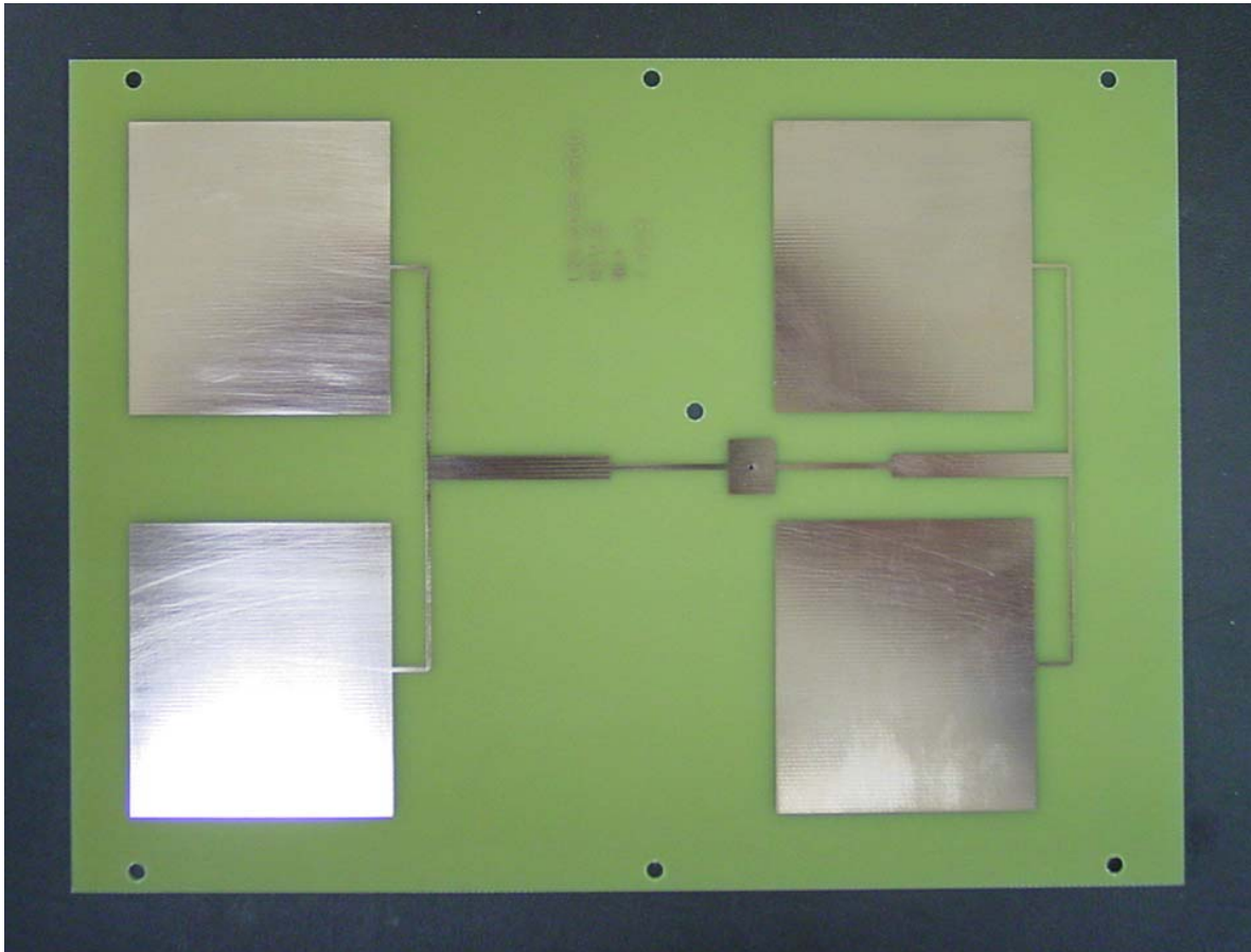
Vertically Polarized Antenna (copper side)
