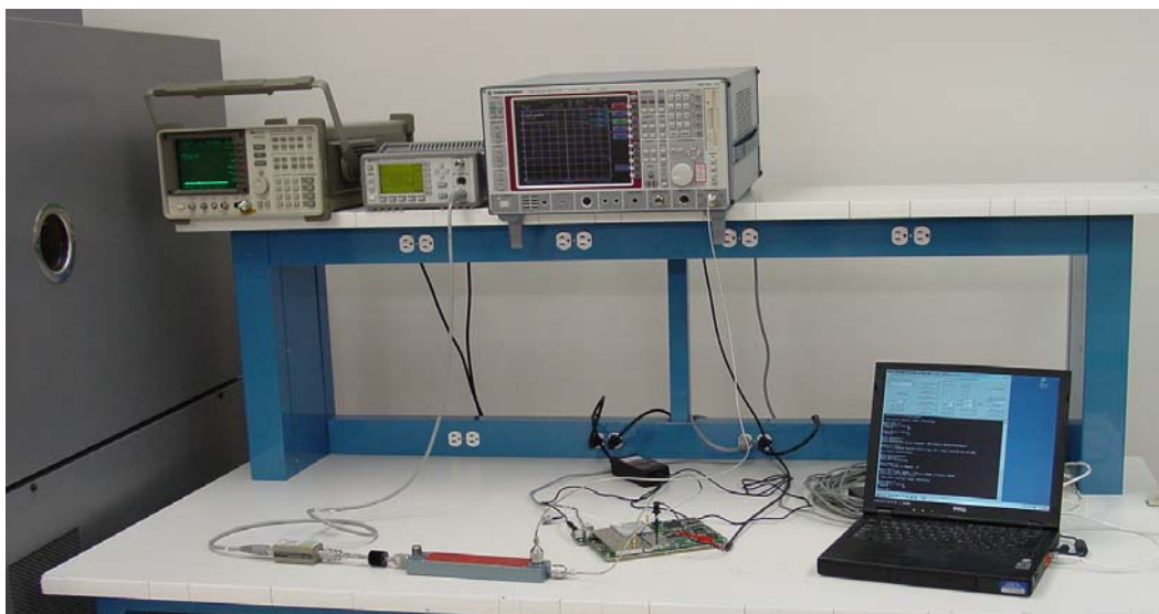
RF Power Out, Modulation Characteristics, Occupied Bandwidth
