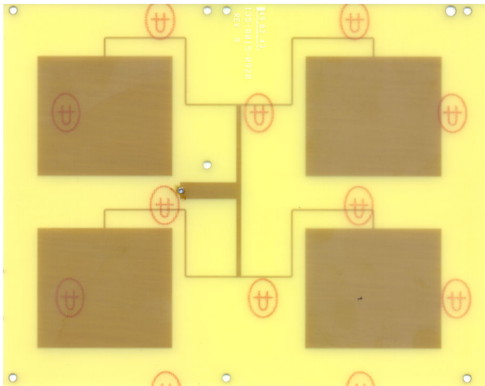
Horizontal Antenna Board, Top Side View
