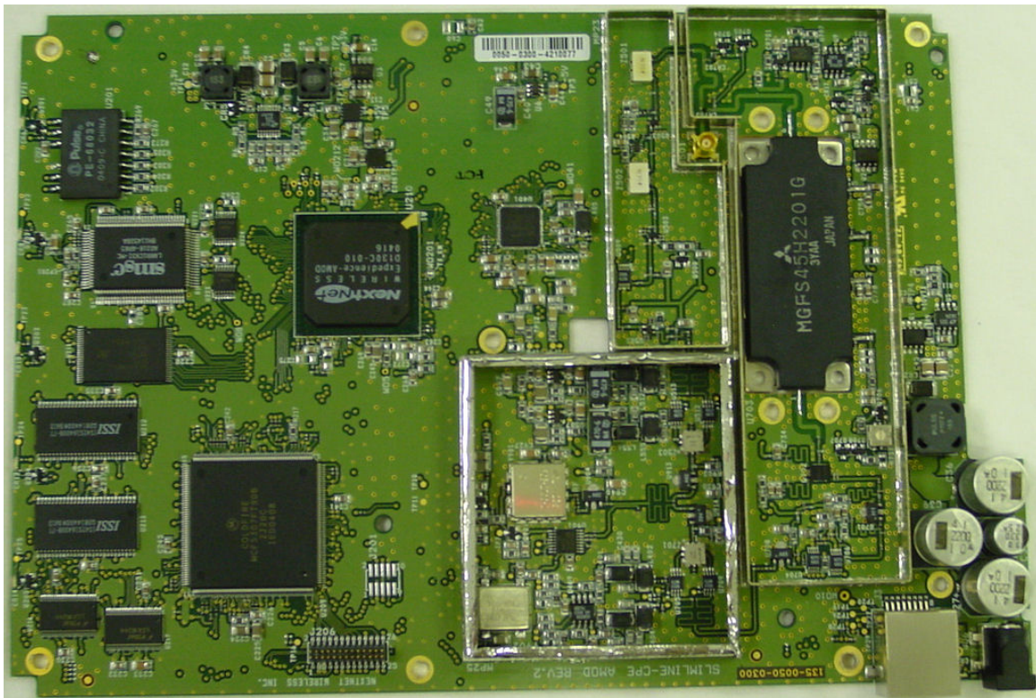
Main Board with Shields Removed, Top Side View
