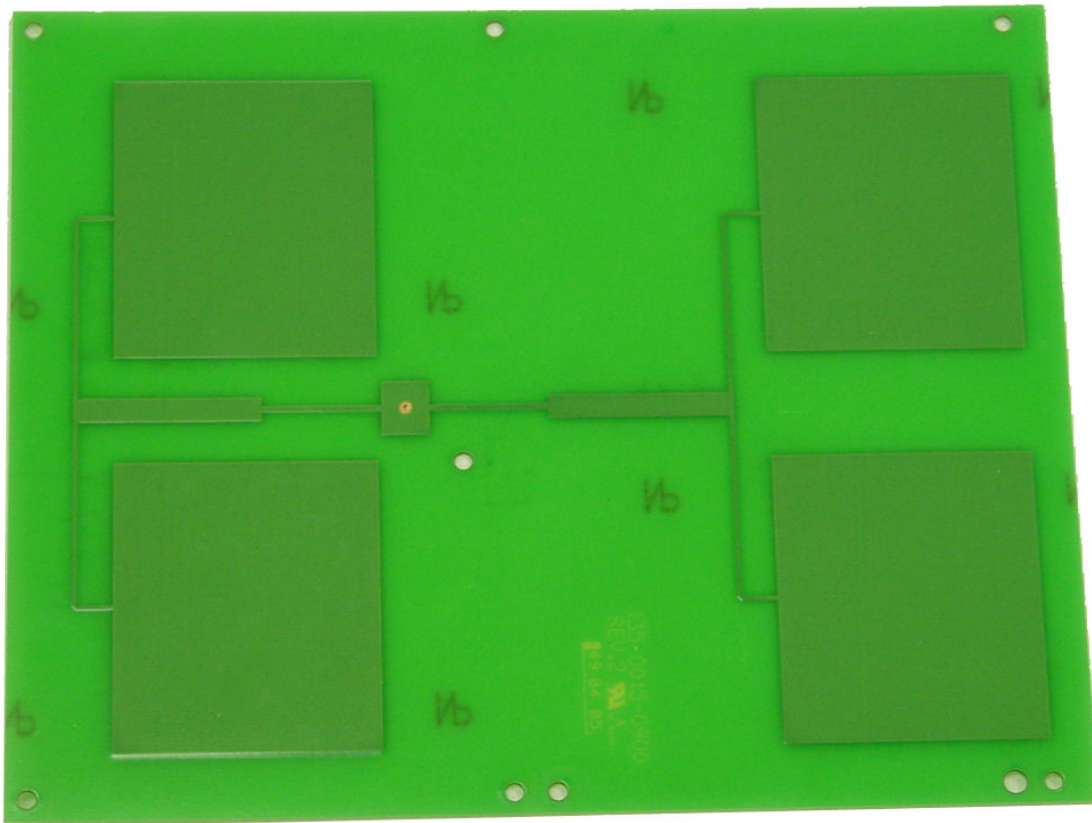
Vertical Antenna Board, Top Side View
