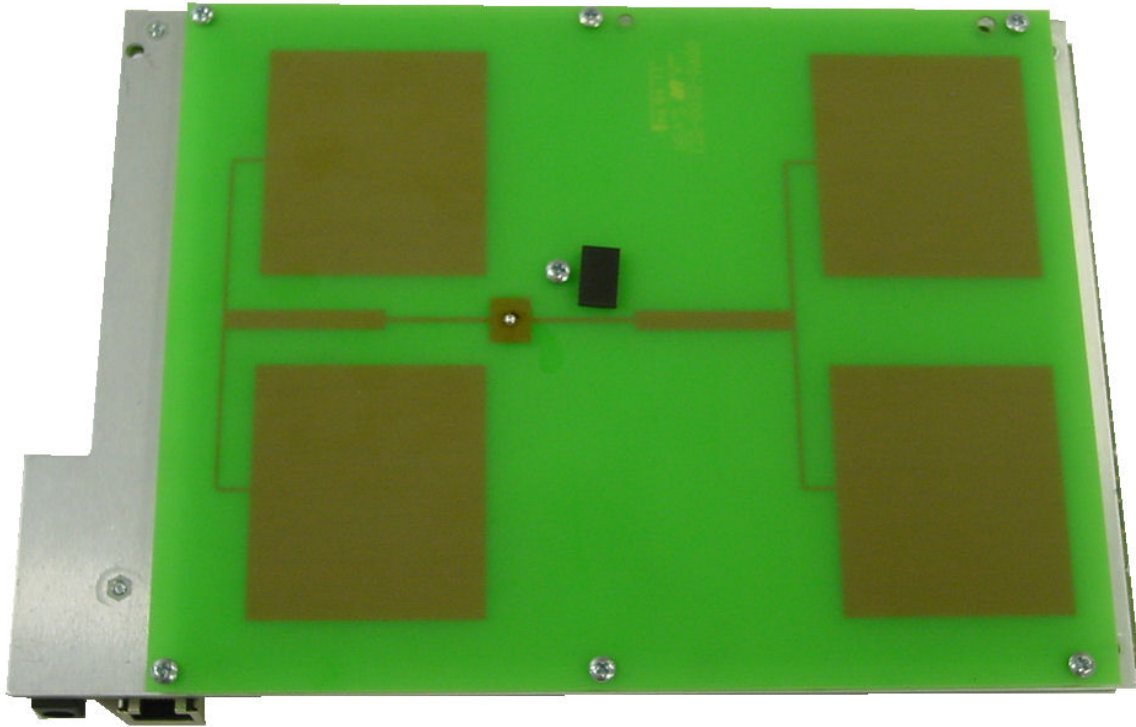
Vertical Antenna Board, Bottom Side View
