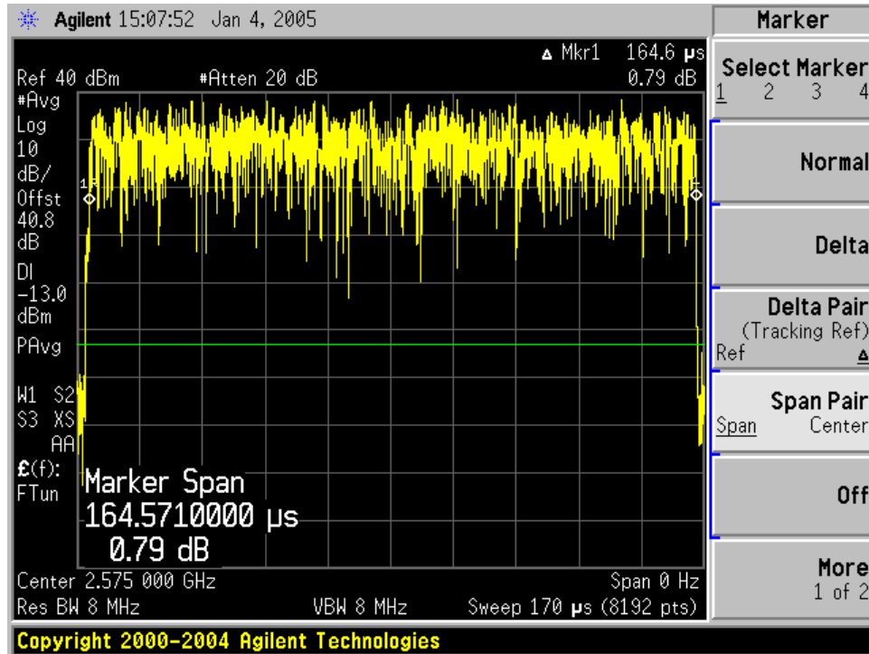
Transmit Pulse Number 1 "On" Time = 164.6 \mu s
