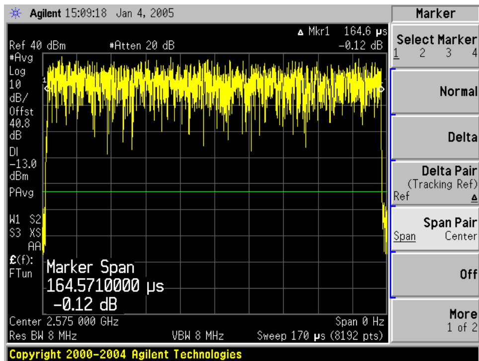
Transmit Pulse Number 2 "On" Time = 164.6 \mu s
