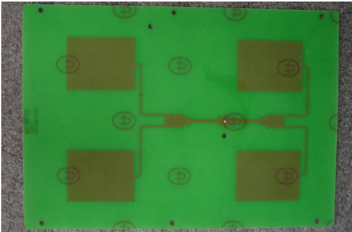
Vertically Polarized Antenna
