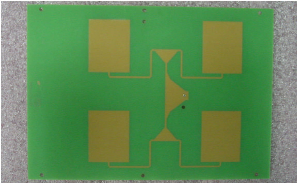
Horizontally Polarized Antenna
