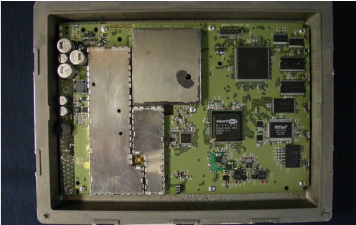
Main Board (component side / with shields)
