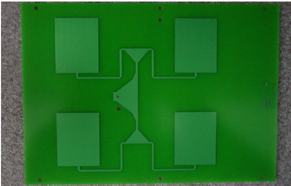
Horizontally Polarized Antenna (copper side)
