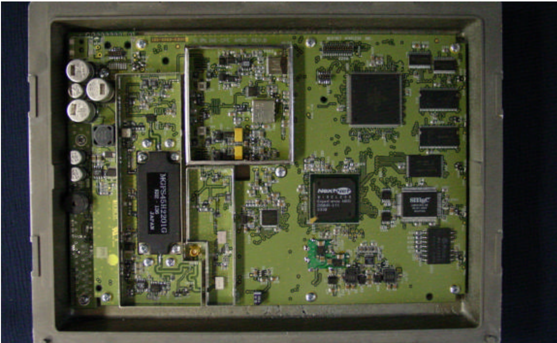
Main Board (component side / no shields)
