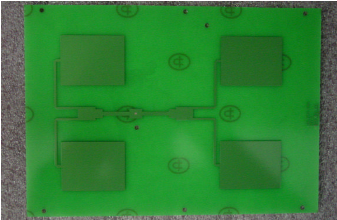
Vertically Polarized Antenna (copper side)
