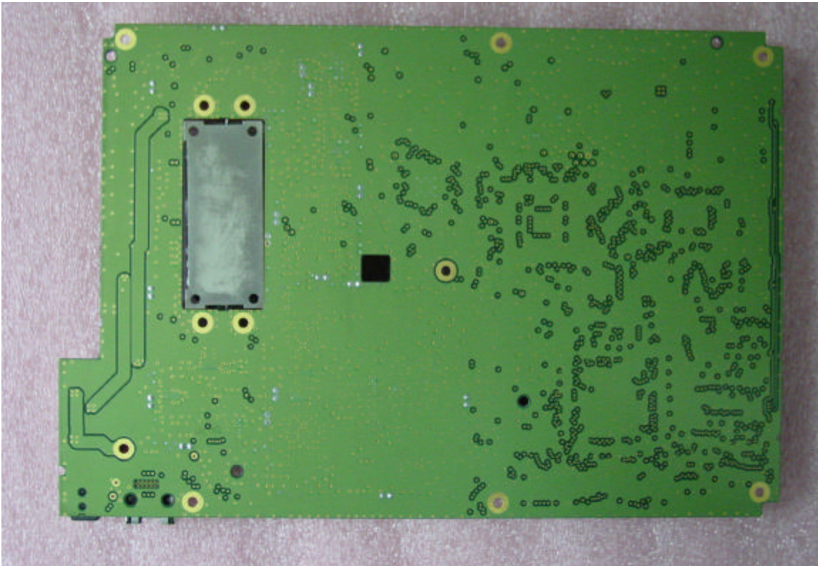
Main Board (back side)
