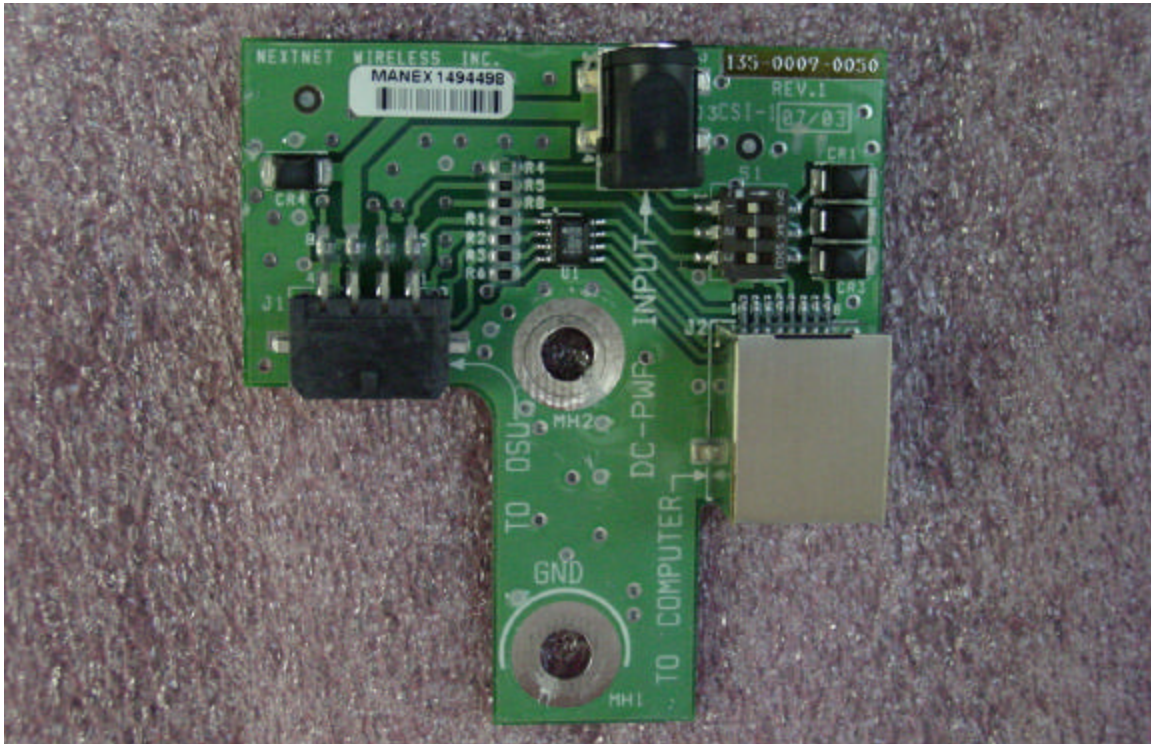
Network Interface Module PCB component side
