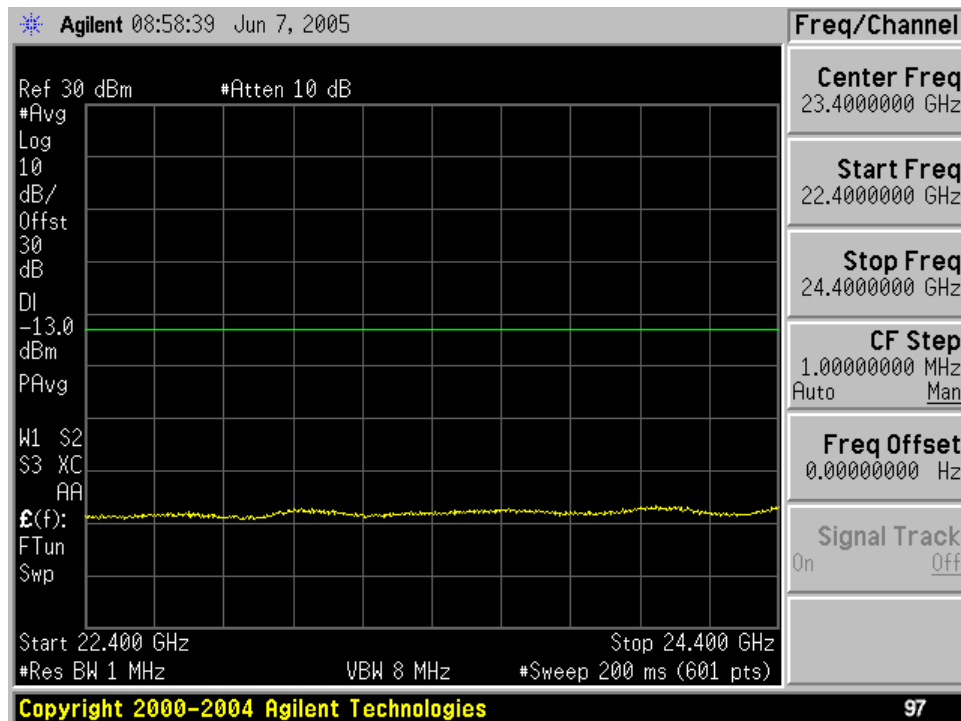
9 th Harmonic of 2687.25 MHz
