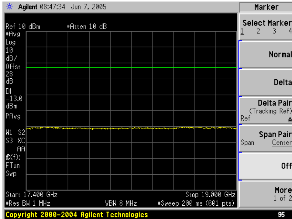
7 th Harmonic of 2687.25 MHz
