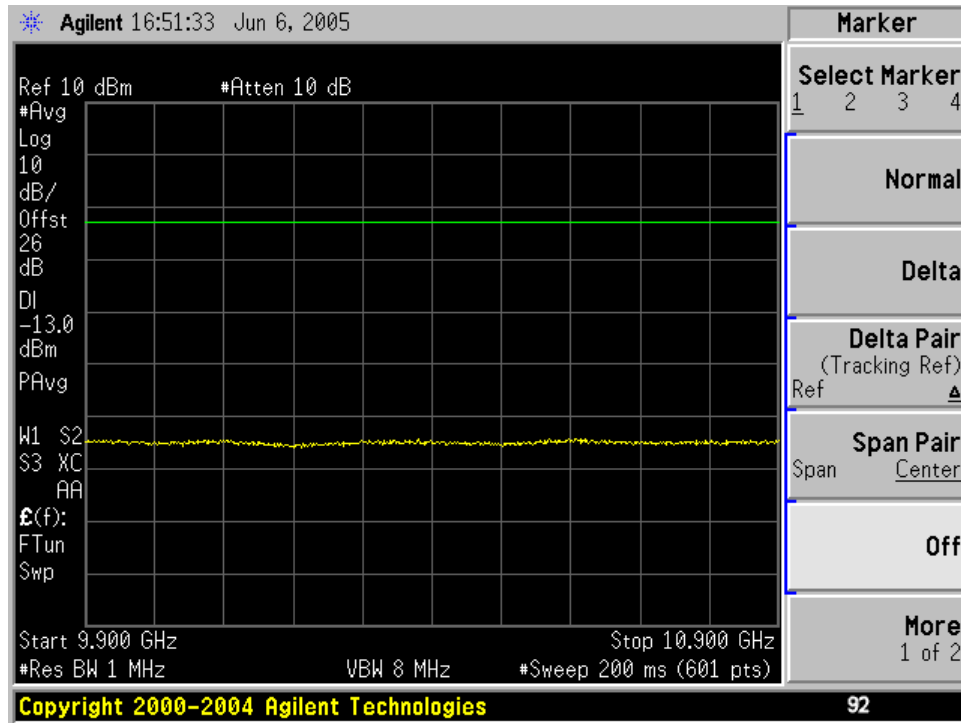
4 th Harmonic of 2687.25 MHz
