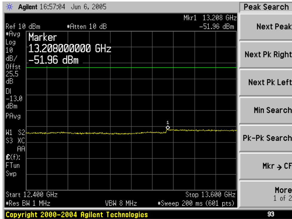
5 th Harmonic of 2687.25 MHz
