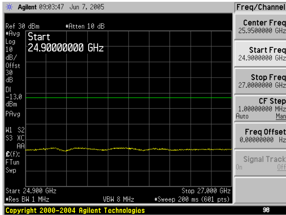
10th Harmonic of 2687.25 MHz
