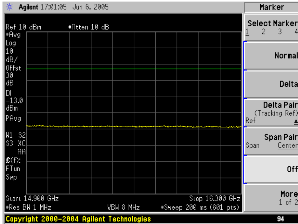
6 th Harmonic of 2687.25 MHz
