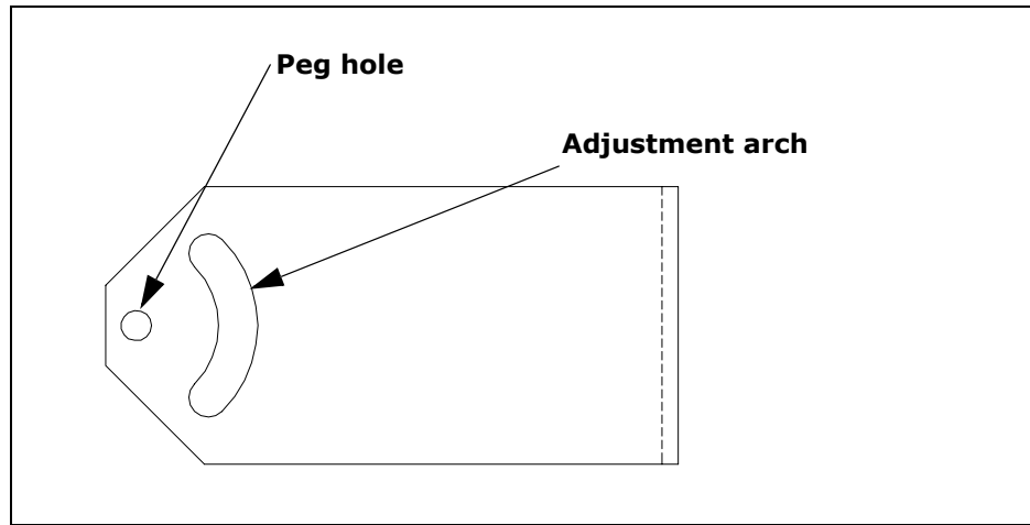
Figure 7 Adjustment arch and peg hole in mounting bracket
