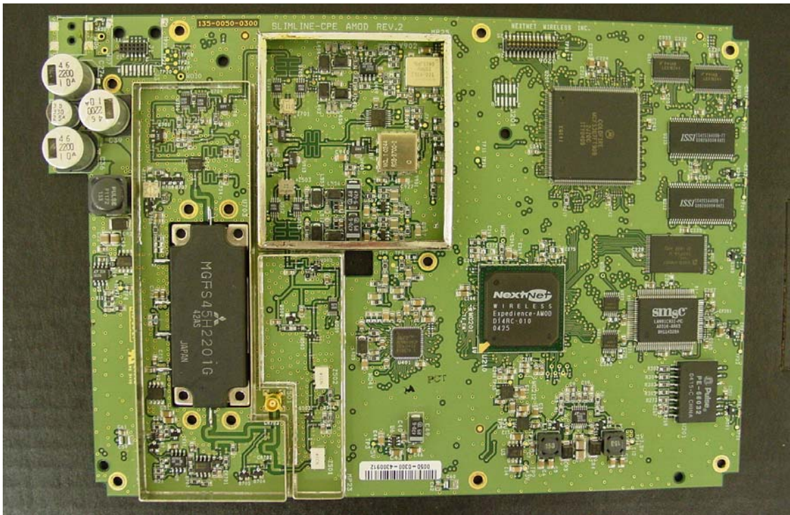
Main PC Board component side (no shields)
