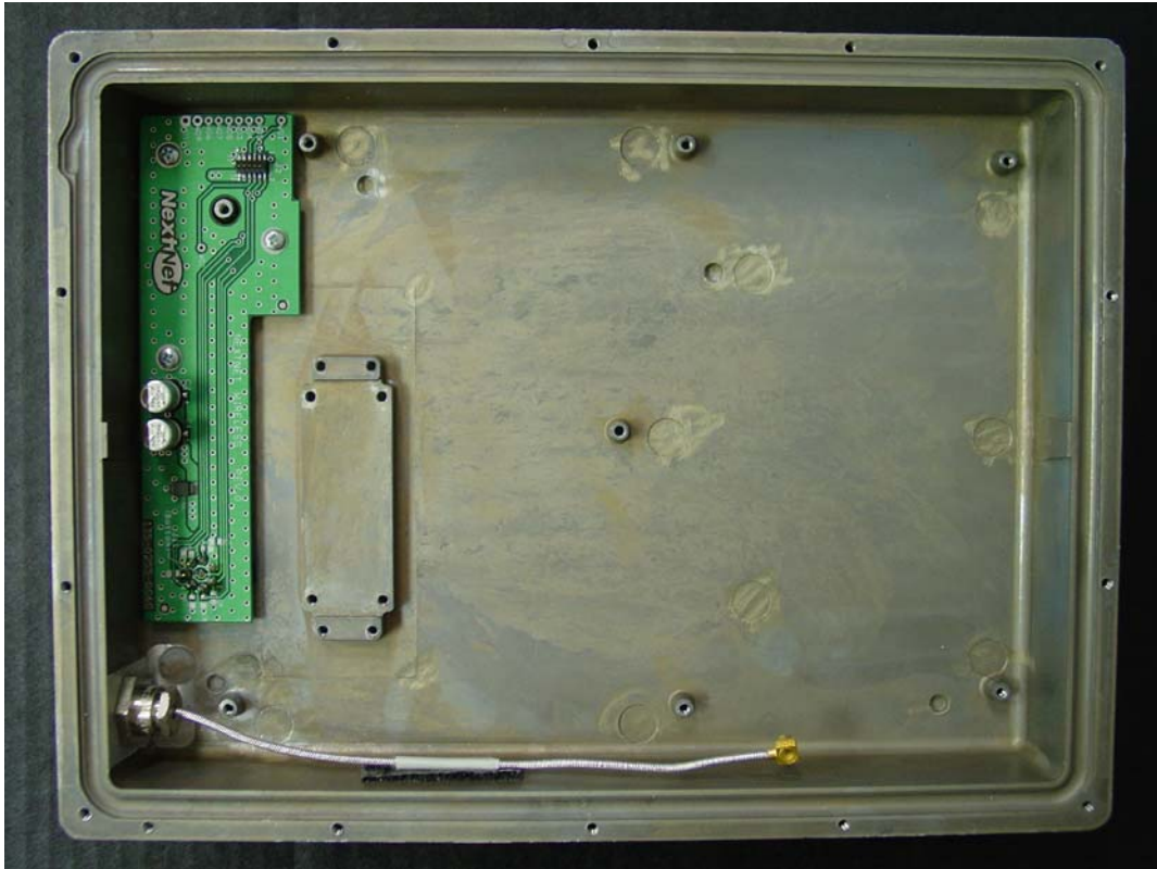
Interface board in casting
