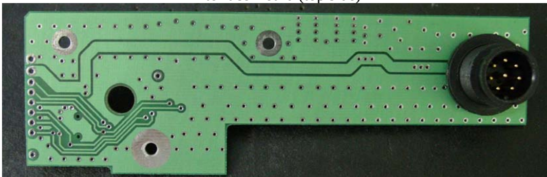
Interface Board (bottom side)
