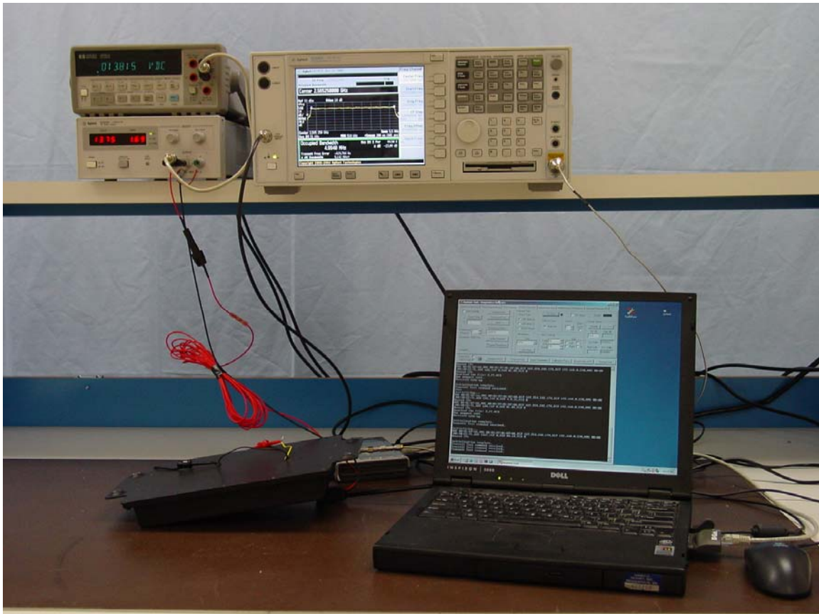
Part 27: RF Power Out, Modulation Characteristics, Occupied Bandwidth, Spurious Emissions at Antenna Terminal (2 watts)
