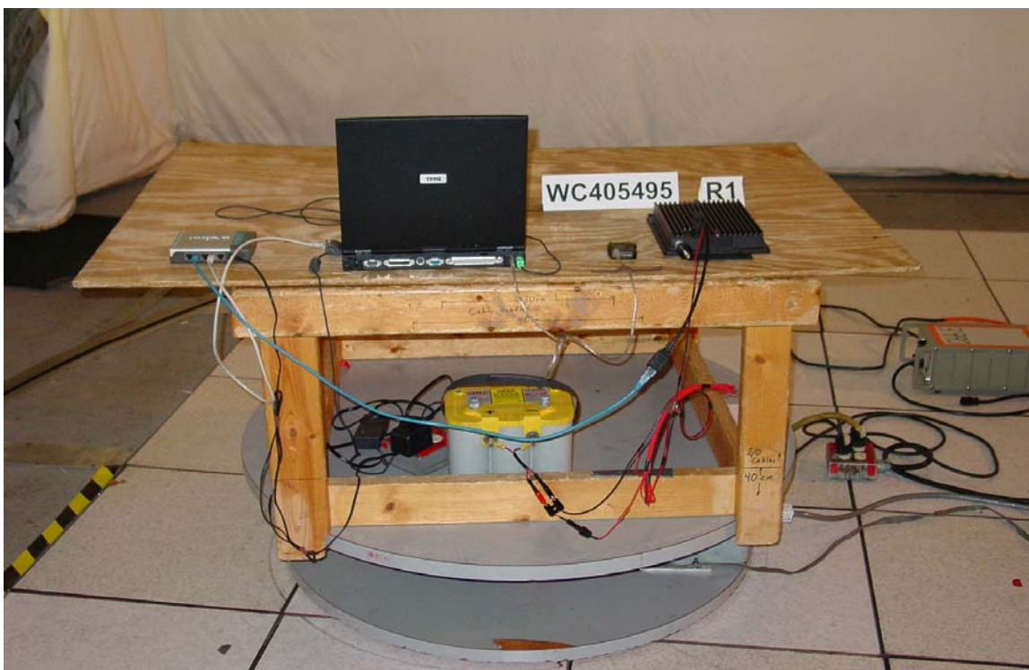
Field Strength of Spurious Radiation (rear view)
