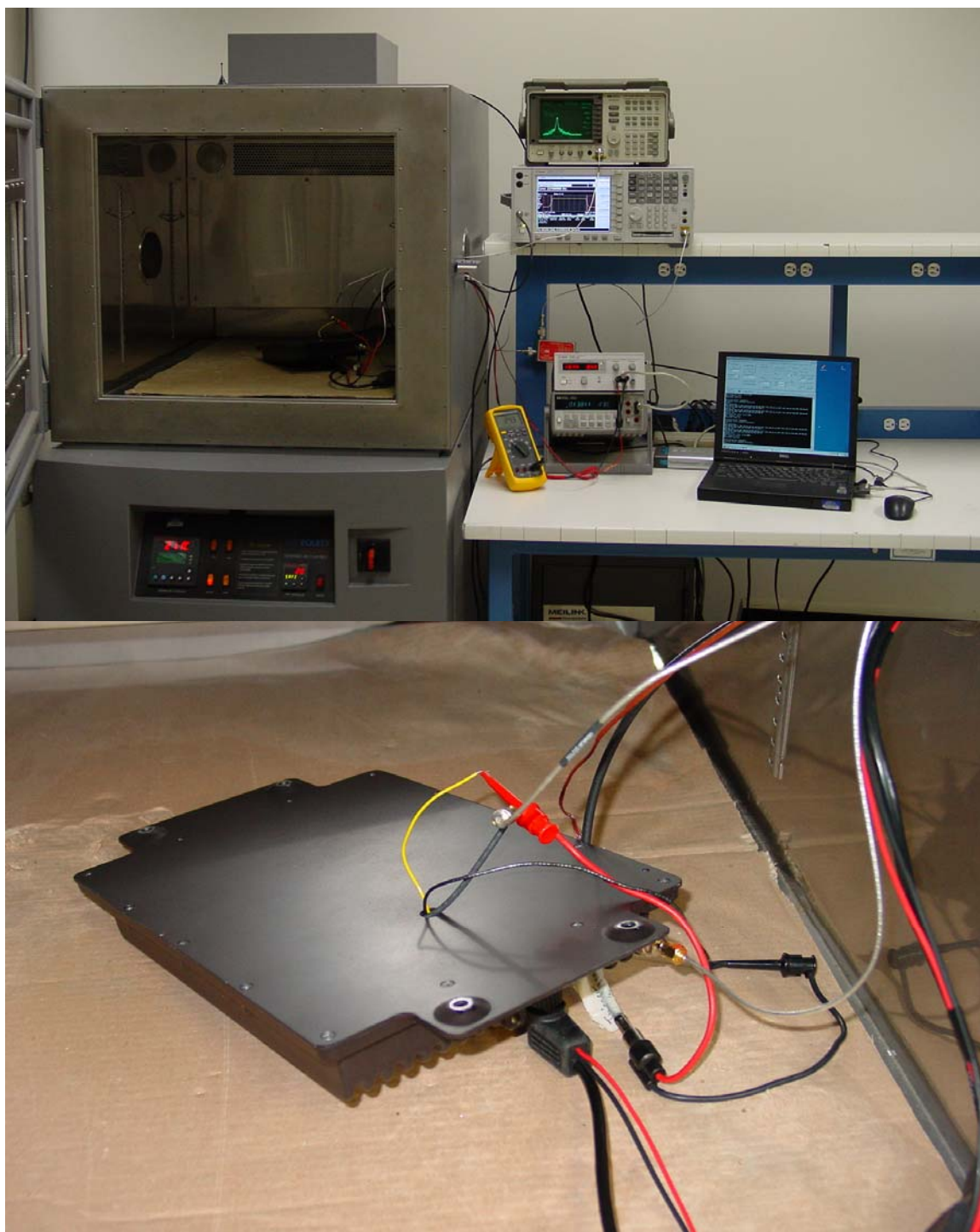
Frequency Stability
