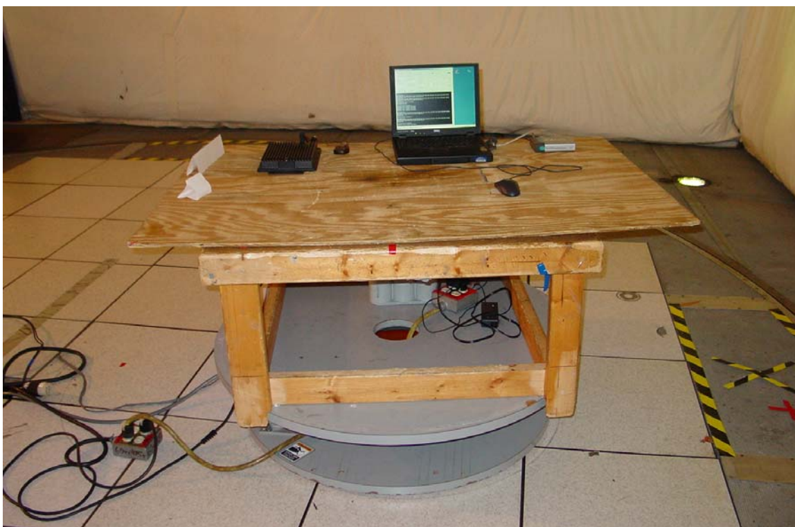
Field Strength of Spurious Radiation (front view)
