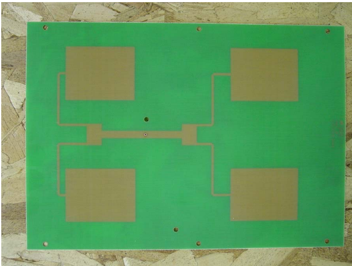
Vertically Polarized Antenna
