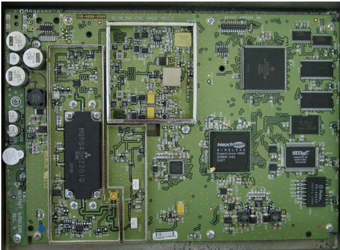
Main PC Board component side (no shields)
