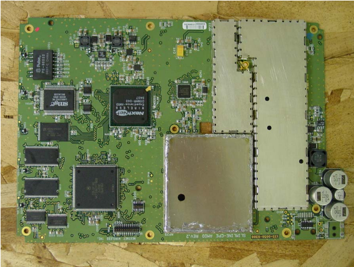
Main PC Board component side (with shields)
