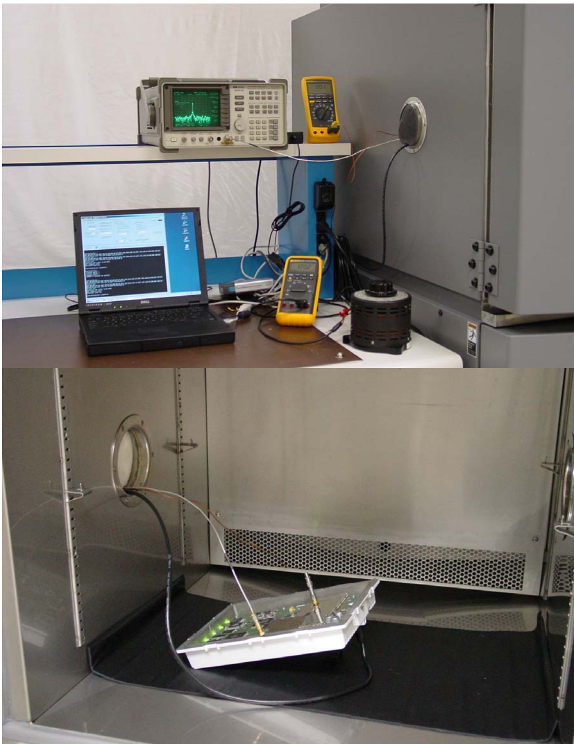
Frequency Stability
