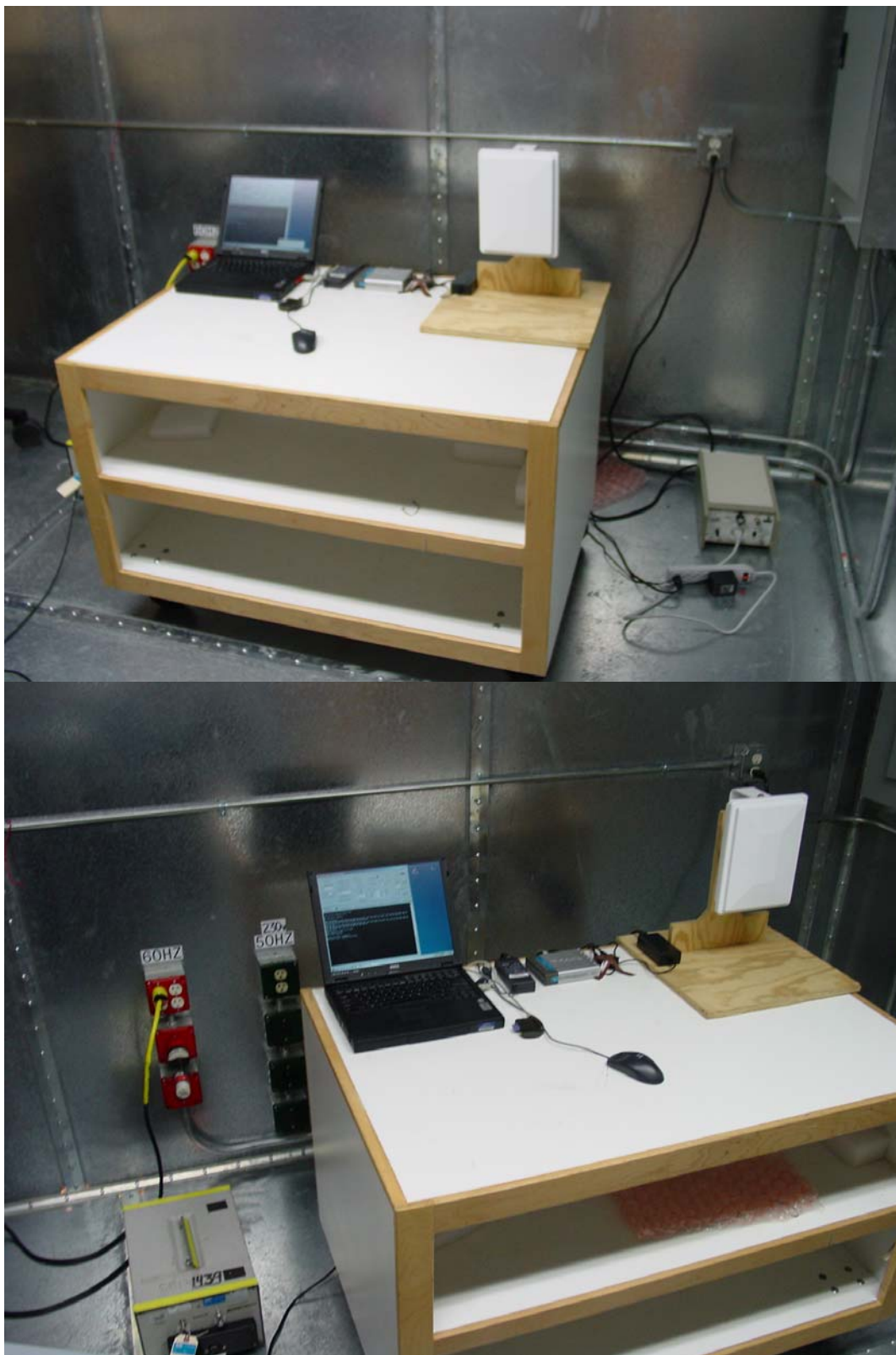
Conducted Emissions (front view)
