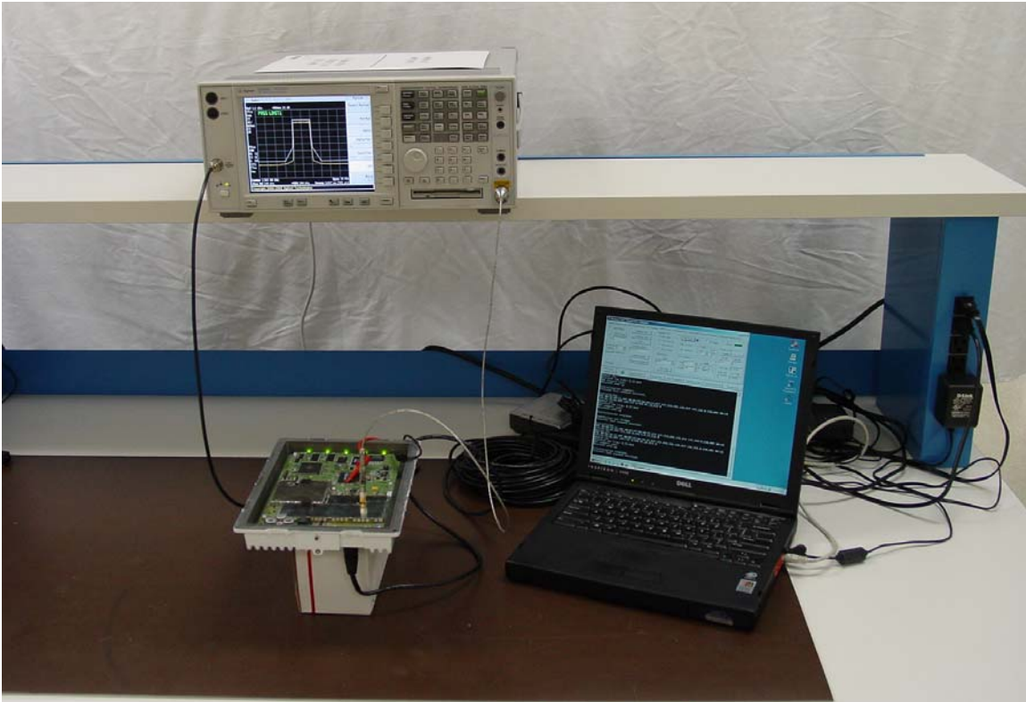
Parts 21/74: Average RF Power Out, Modulation Characteristics, Occupied Bandwidth, Spurious Emissions at Antenna Terminal (2 watts)
