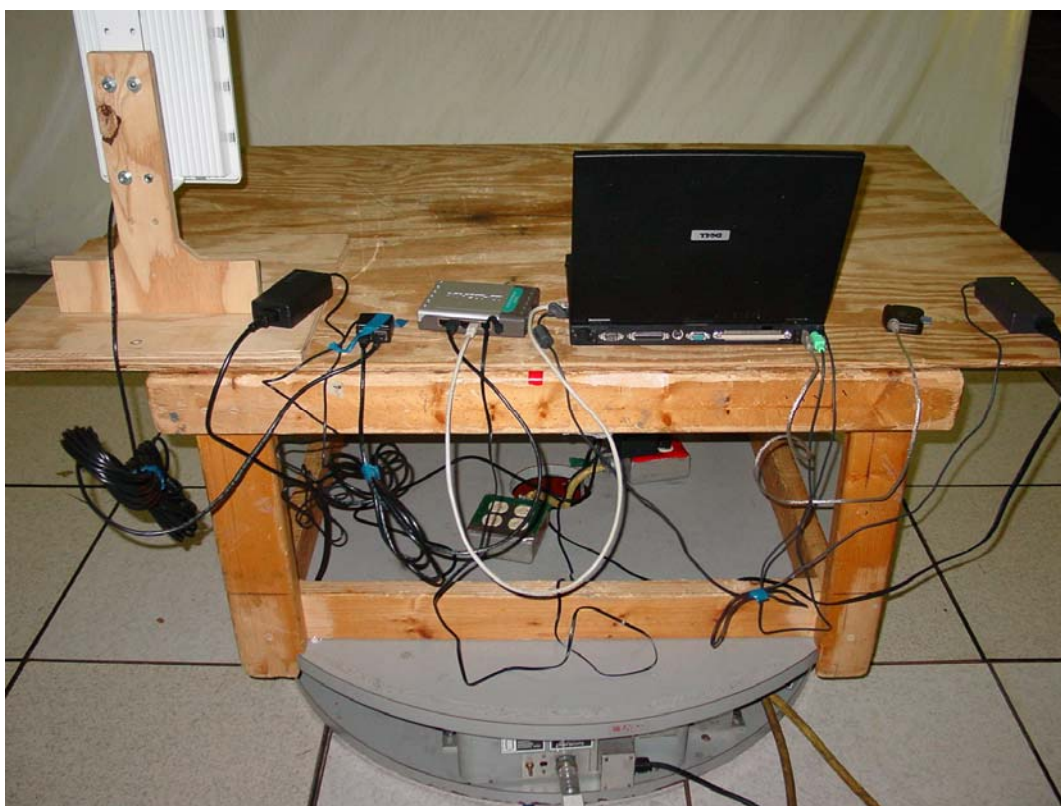
Field Strength of Spurious Radiation (rear view)
