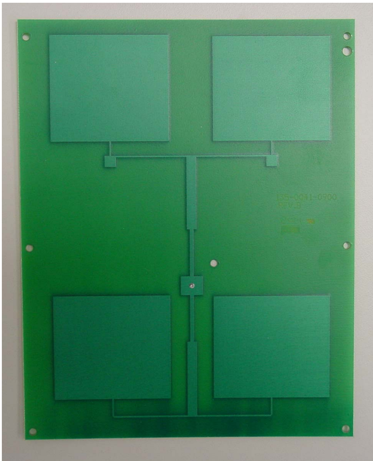
Vertically Polarized Antenna (copper side)
