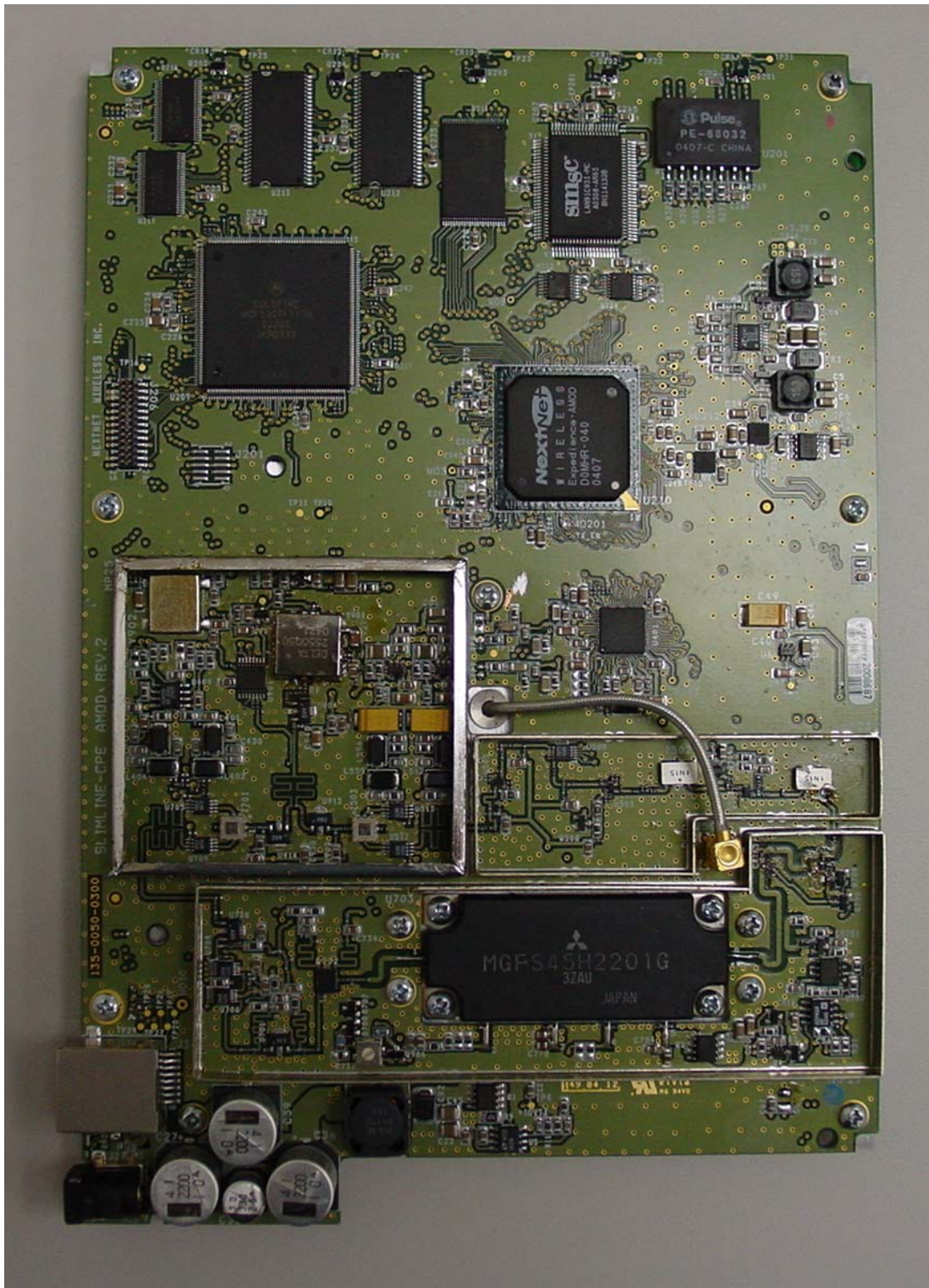
RF Board component side (no shields)
