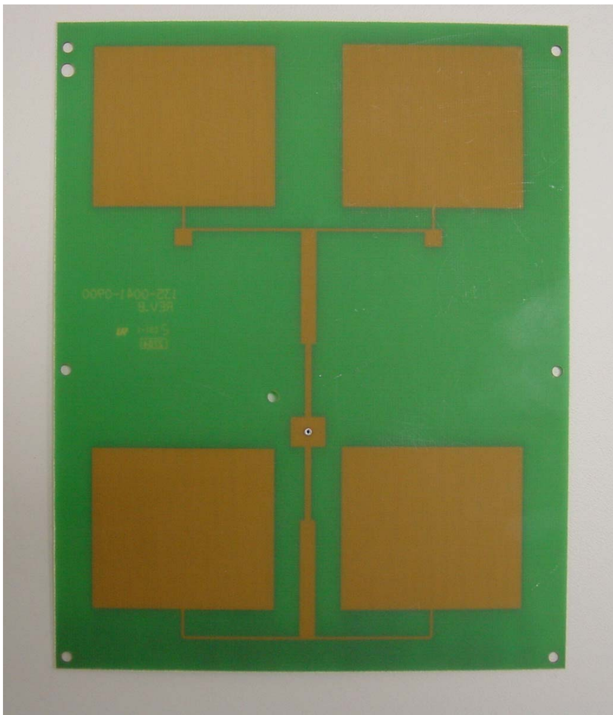
Vertically Polarized Antenna
