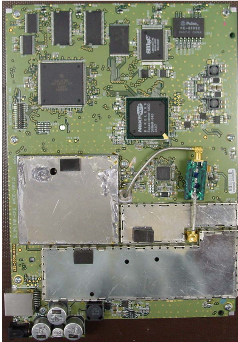
RF Board, Low Pass Filter component side (with shields)
