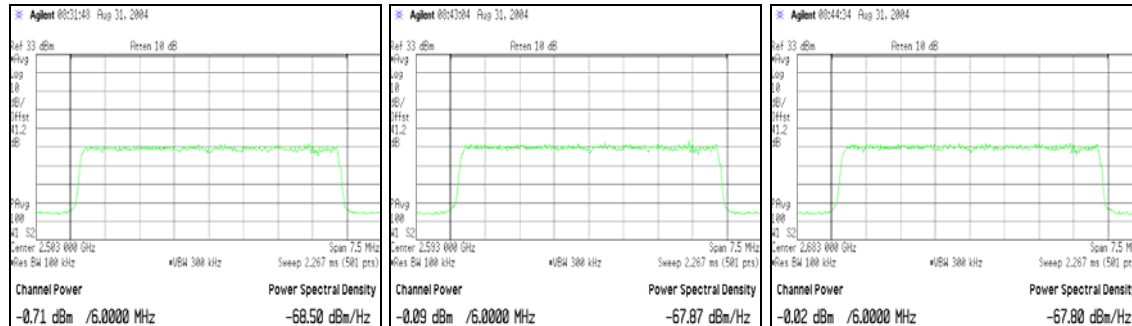
4-QAM 2503 MHz
