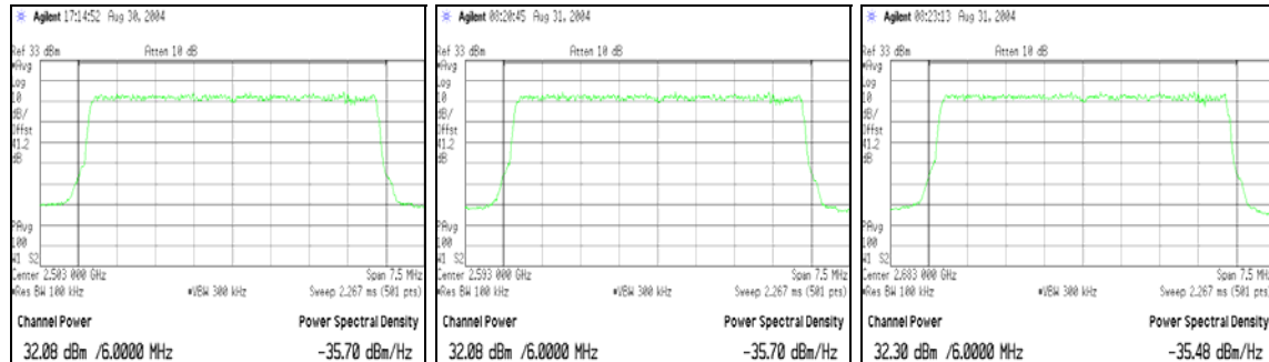
4-QAM 2503 MHz
