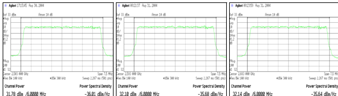
64-QAM 2503 MHz
