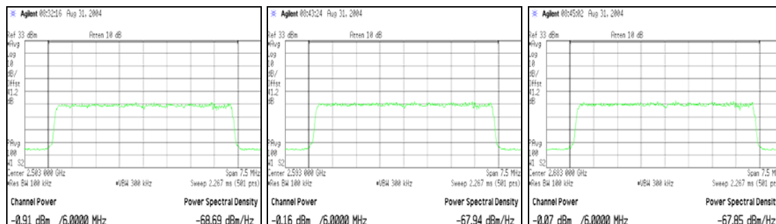
16-QAM 2503 MHz
