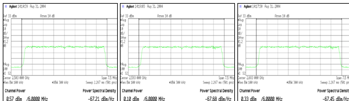
64-QAM 2503 MHz
