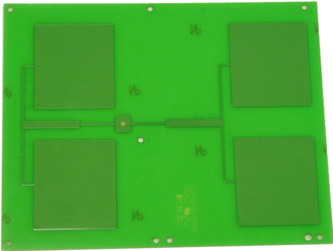
Vertical Antenna Top Side View
