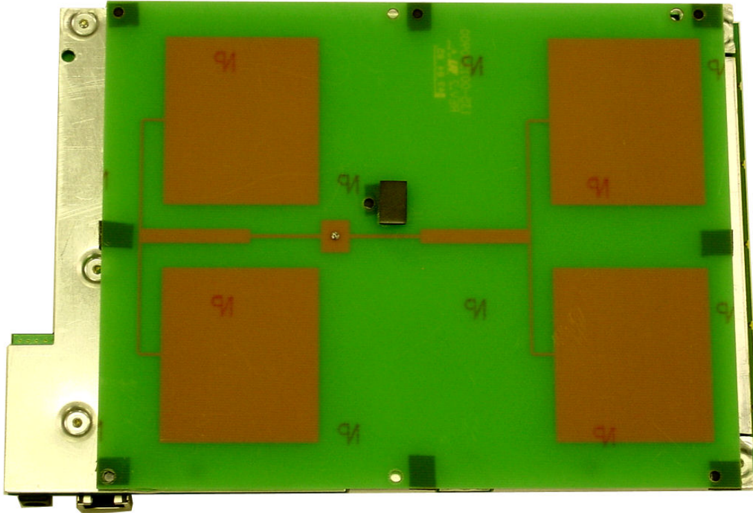
Vertical Antenna Bottom Side View
