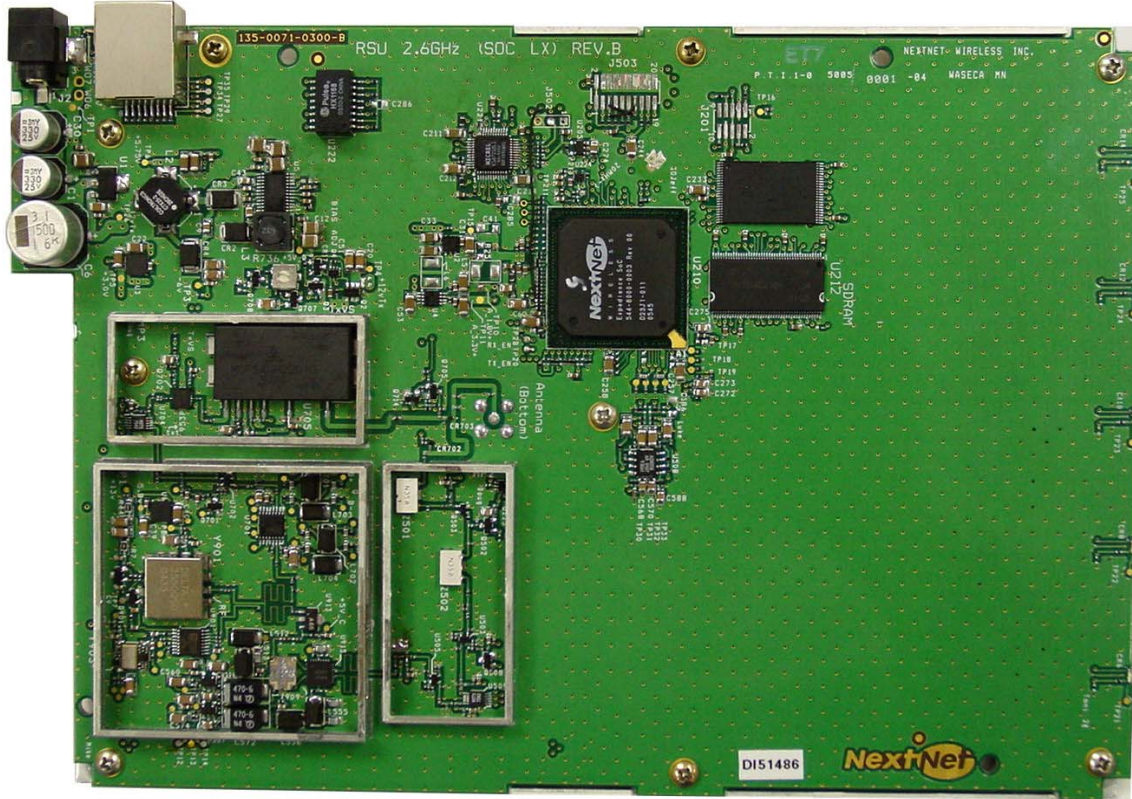
Main PC Board Component Side View (Without Shields)
