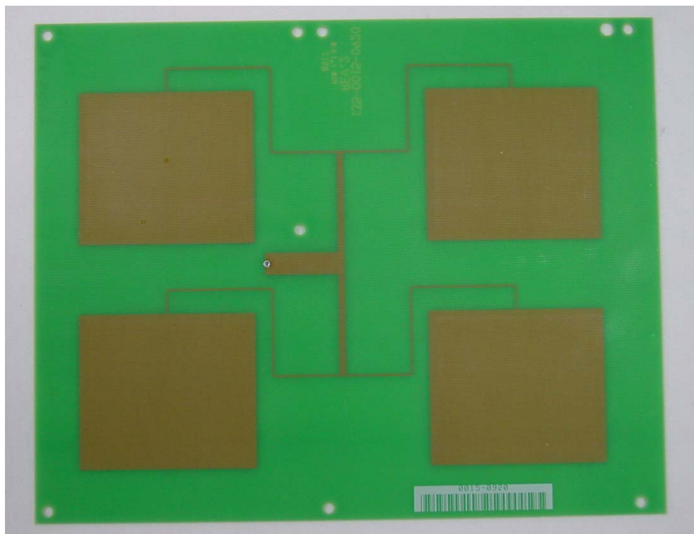
Horizontal Antenna Bottom Side View
