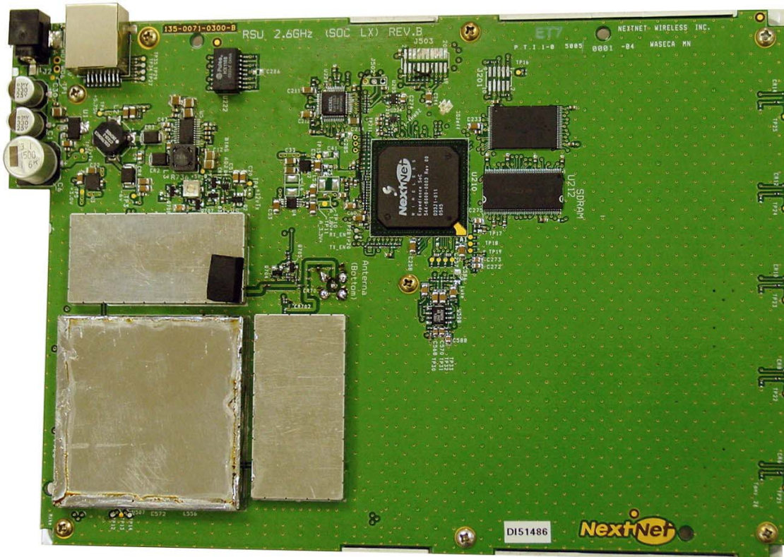
Main PC Board Component Side View (With Shields)
