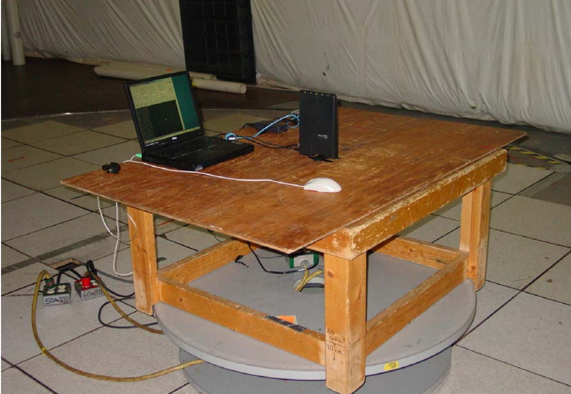
Field Strength of Spurious Radiation (Front View)
