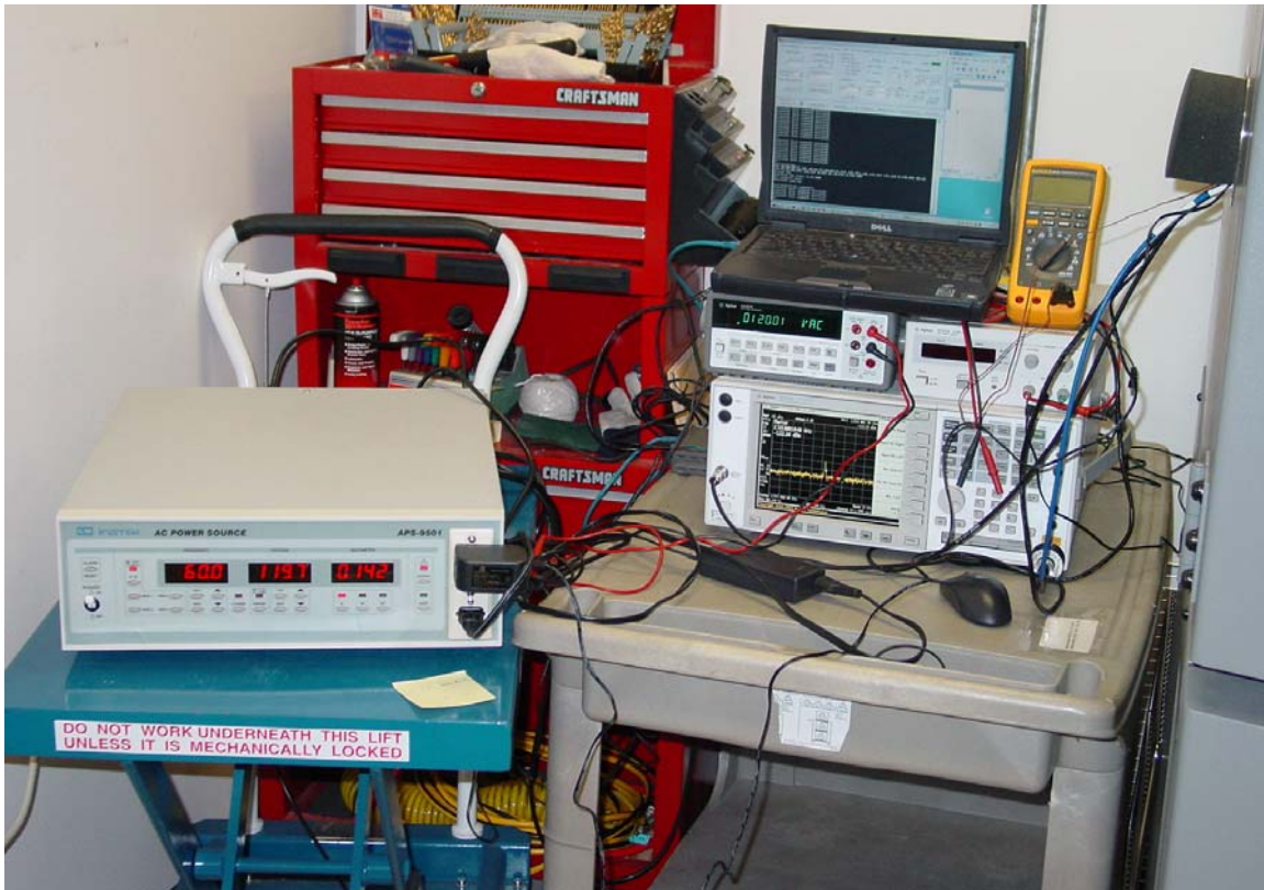
Frequency Stability Test Setup
