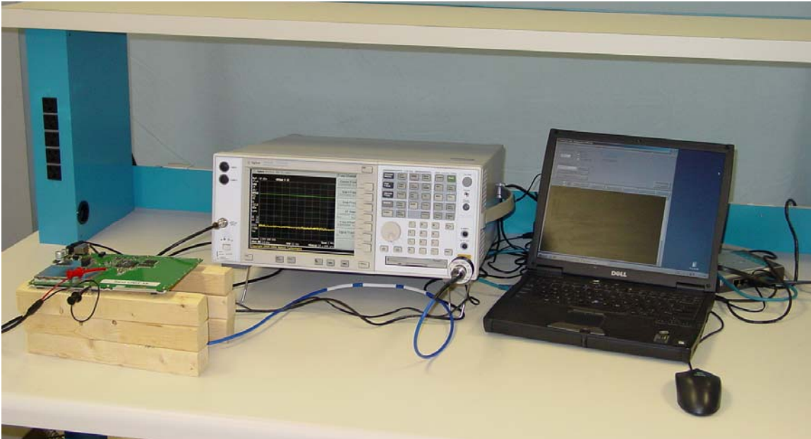
Test Bench Setup
