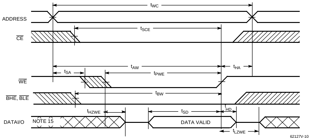
Write Cycle No.3 ( \overline{WE} Controlled, \overline{OE} LOW) [13, 14]
