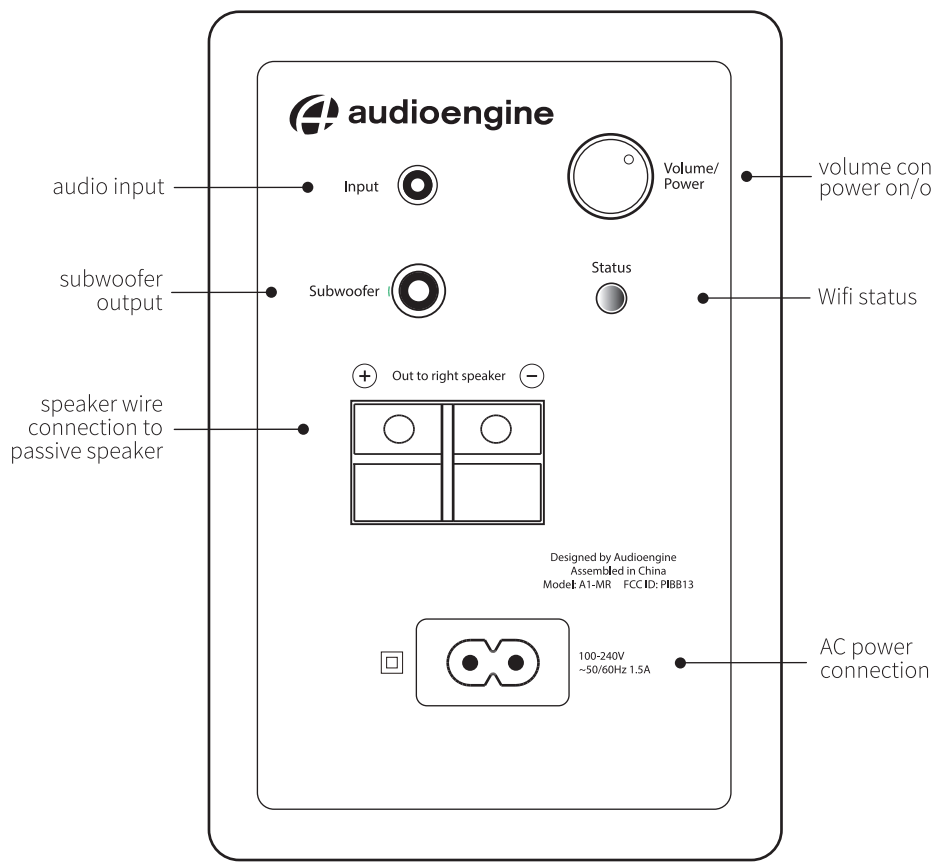
A1 powered (left) speaker - rear panel
