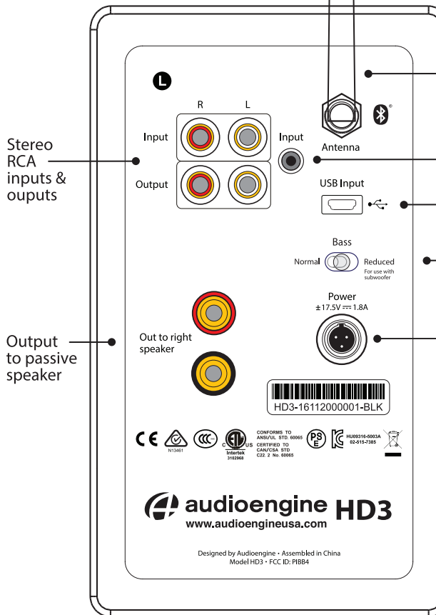
HD3 powered (left) speaker - rear panel
