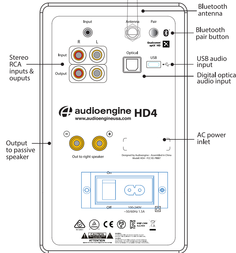
HD4 powered (left) speaker - rear panel
