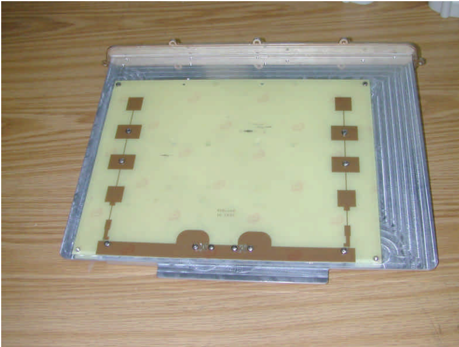
BSR antenna
