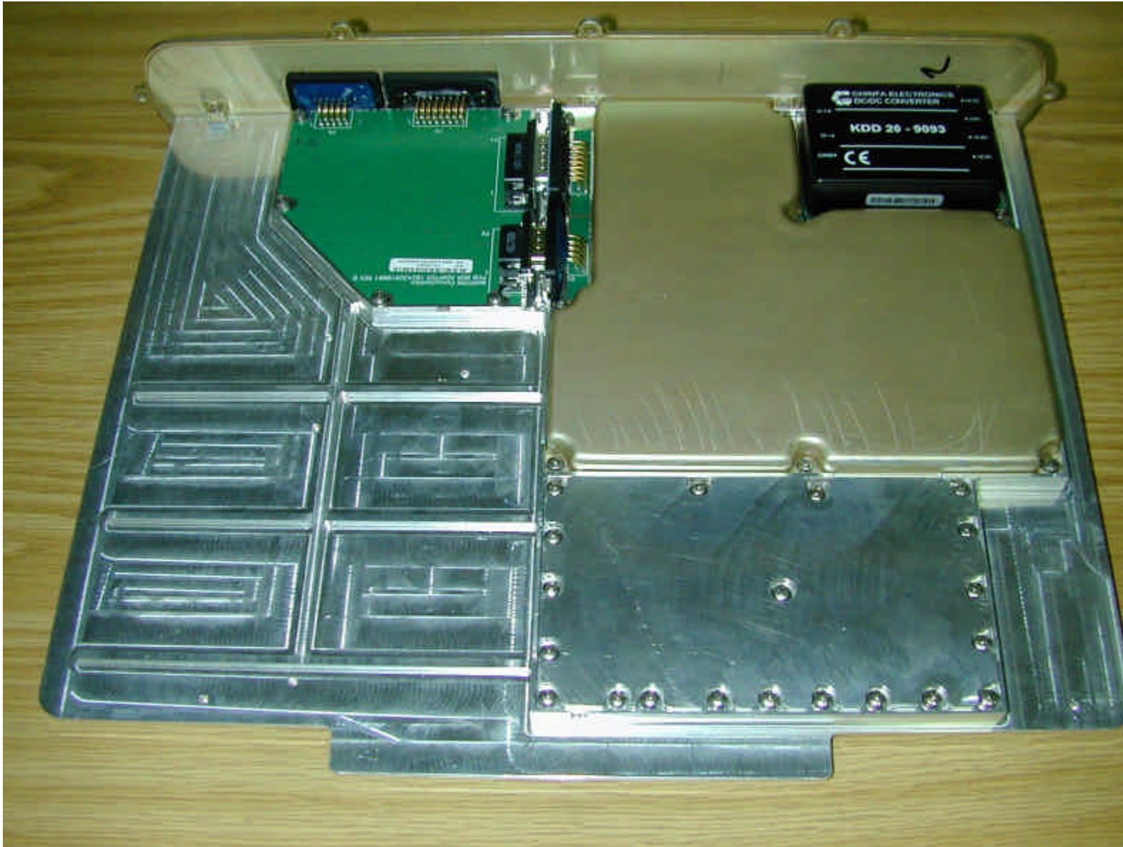
BSR with cover removed
