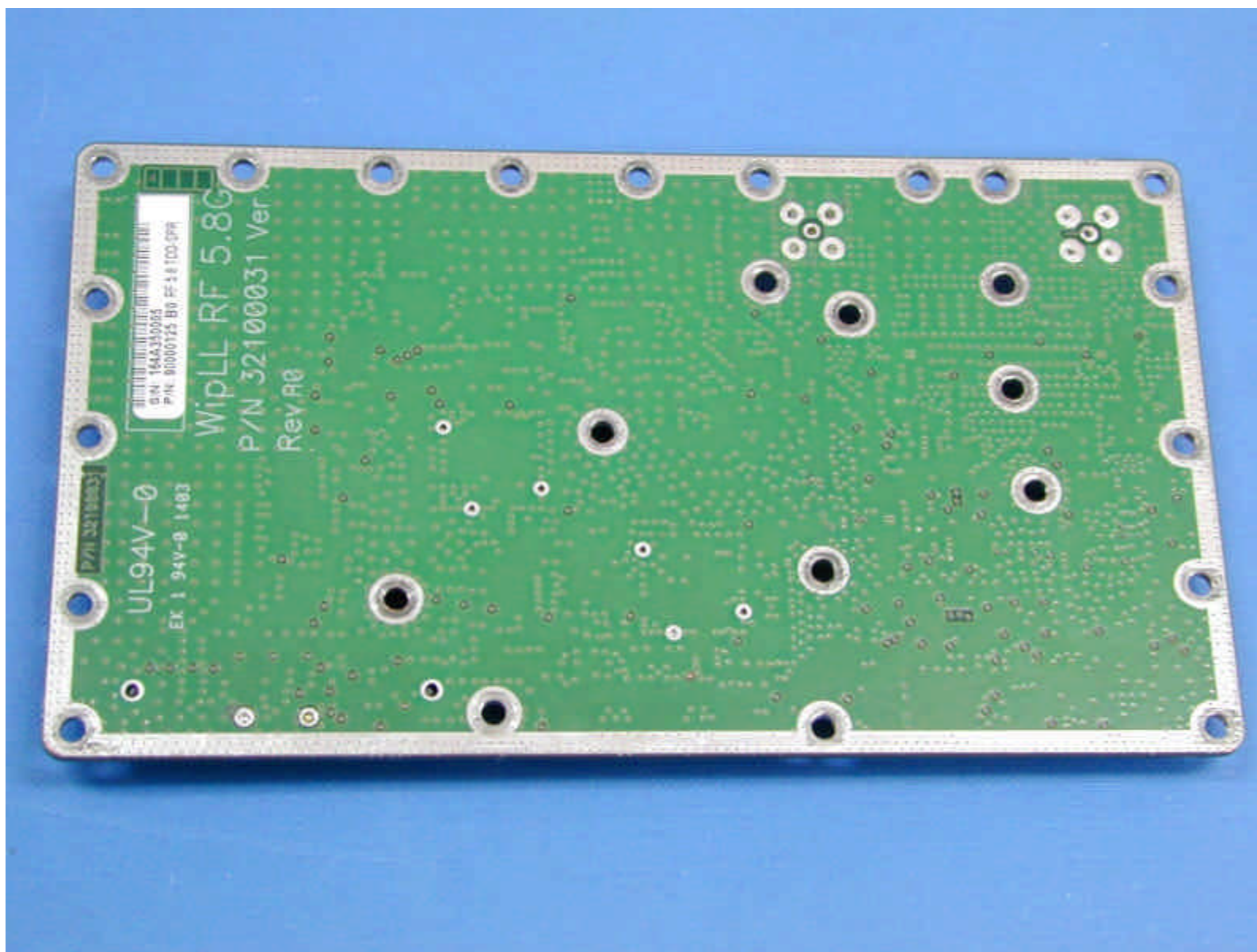
RF PCB for BSR and SPR, second side
