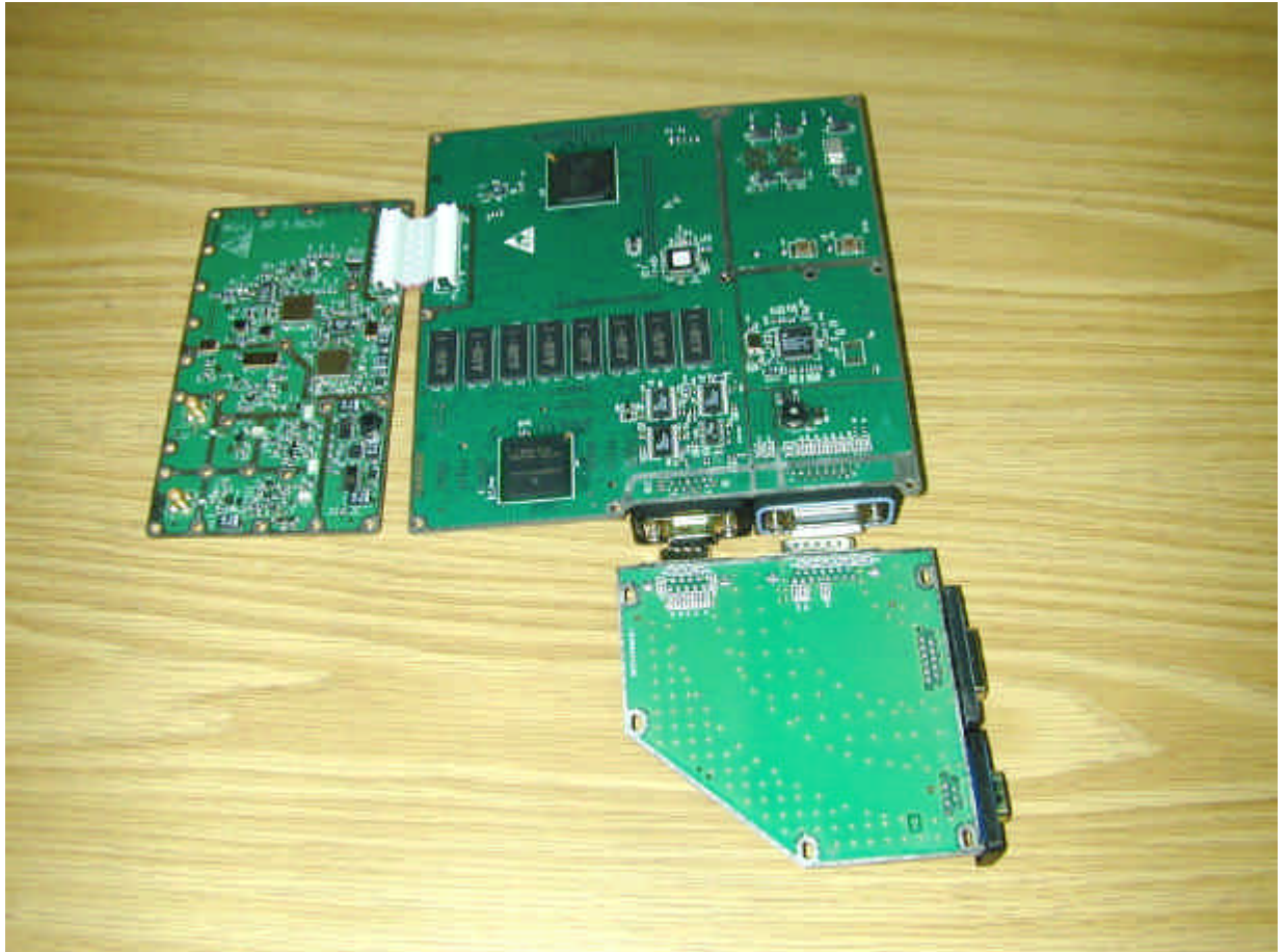
Photograph No.5 BSR 900 MHz RF and digital boards Second side view
