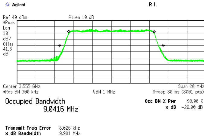
Plot 7.3.2 Occupied bandwidth test result at low frequency
