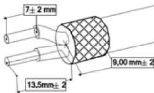
Figure 40: Stripping Dimensions (DC Cable)
