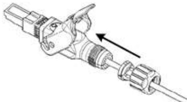
Figure 24: Insert Gland
