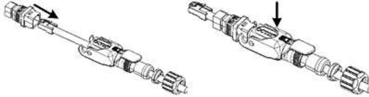
Figure 33: Insert Holder onto RJ45
