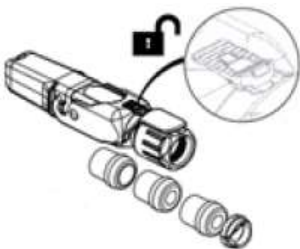
Figure 41: Open Housing Lock
