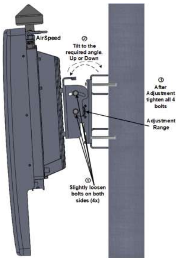
Figure 11: Tilt Adjustment
