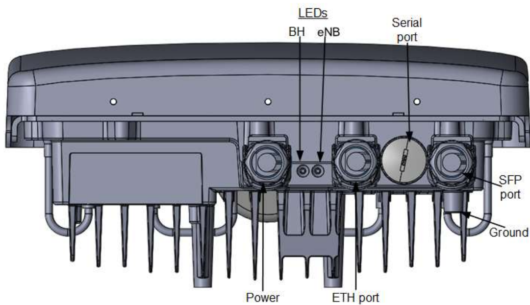
Figure 5: AirSpeed 1030 B48 Bottom Ports
