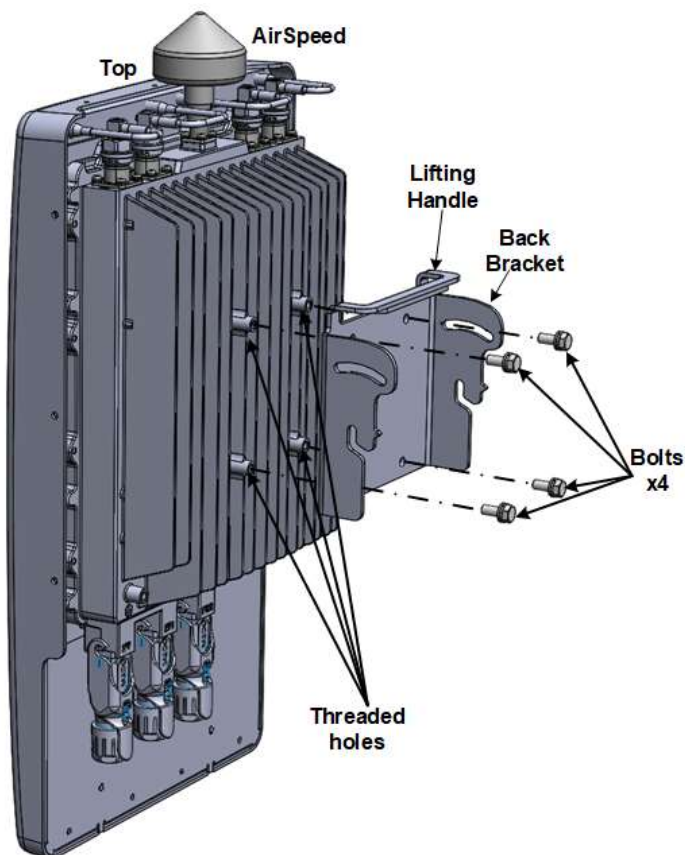
Figure 6: Back Bracket Assembly
