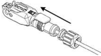
Figure 18: Pass Cable thru Housing
