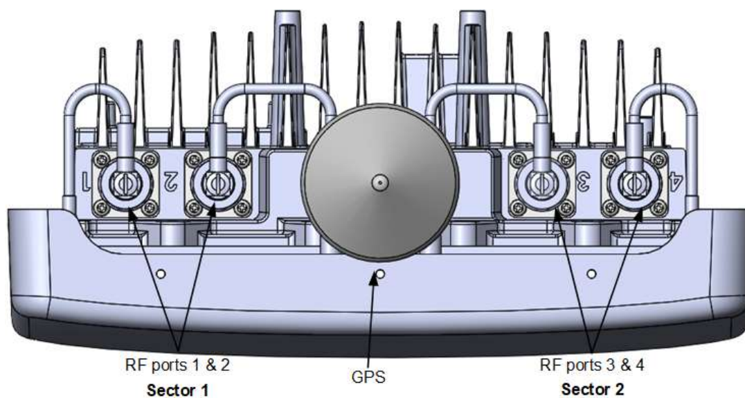
Figure 4: AirSpeed 1030 B48 Top Ports
