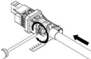
Figure 45: Tighten Two (2) Set Screws
