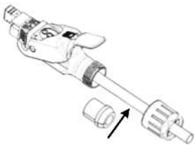
Figure 48: Place Split Rubber Gland
