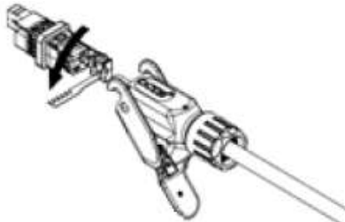
Figure 44: Pass DC Cable Thru
