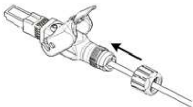
Figure 25: Insert Cone
