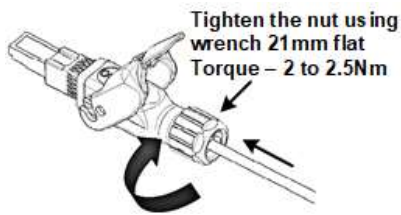
Figure 26: Tighten Gland Nut
