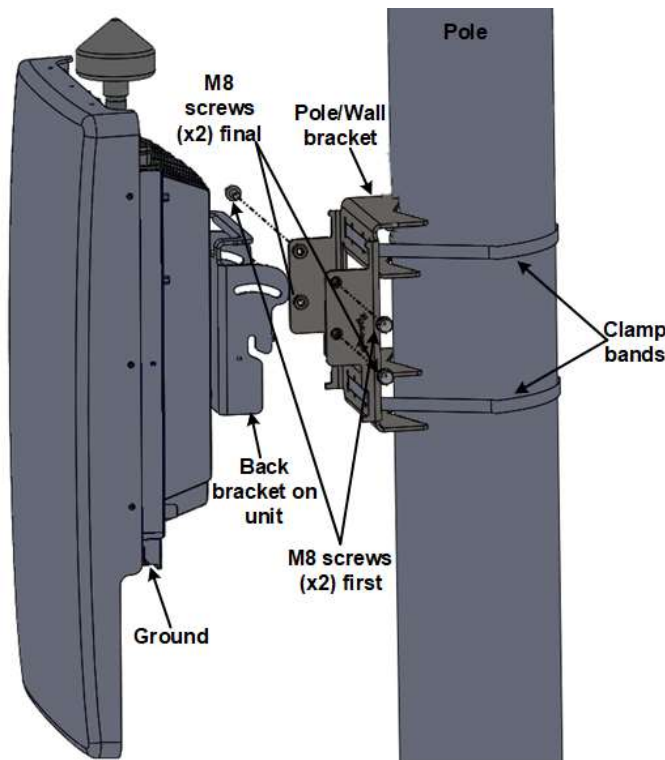
Figure 8: Pole Mounting Assembly
