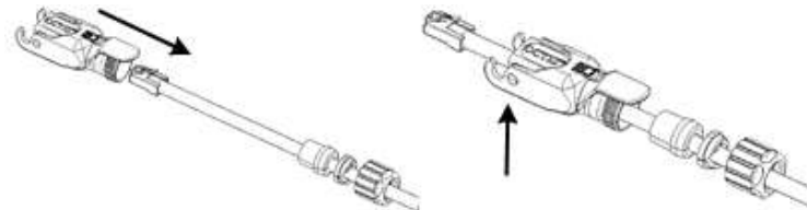
Figure 32: Insert Housing onto Cable
