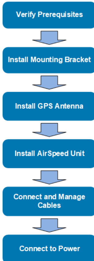
Figure 3: Workflow
