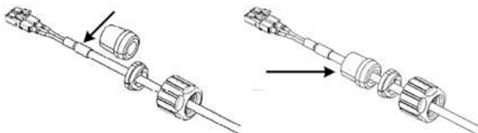
Figure 17: Insert Rubber Gland on Cable
