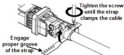
Figure 46: Tighten the Strap Clamp
