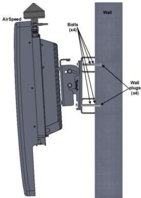
Figure 10: AirSpeed on Wall
