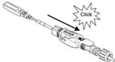
Figure 21: Holder into Housing Base
