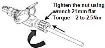
Figure 38: Tighten Gland Nut
