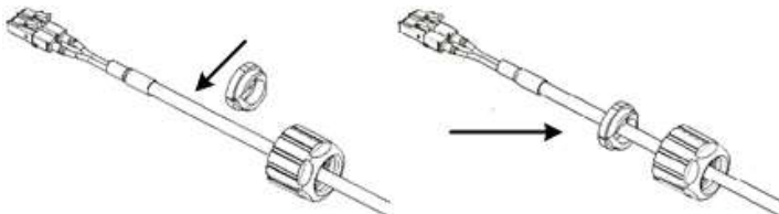
Figure 16: Insert Tightening Cone on Cable
