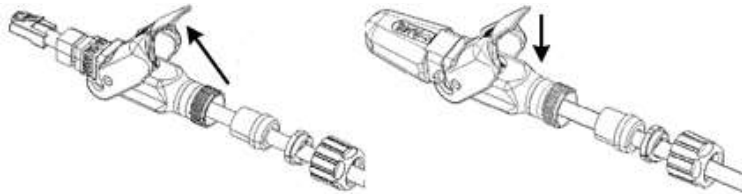
Figure 35: Align RJ45 into Holder
