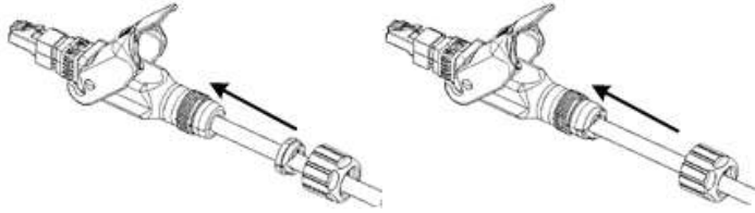
Figure 37: Insert Gland
