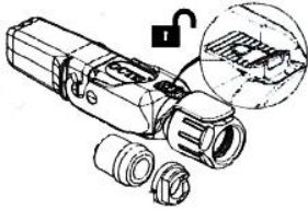
Figure 14: Open Housing Lock
