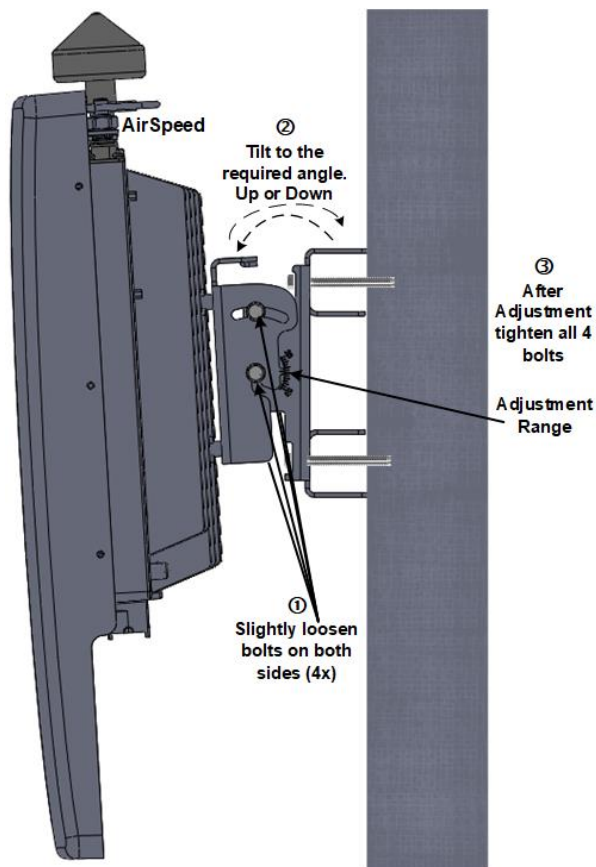
Figure 11: Tilt Adjustment
