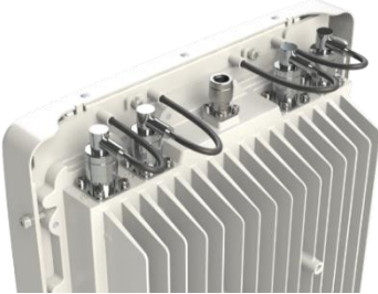
Figure 52: Antenna RF Cables
