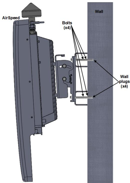
Figure 10: AirSpeed on Wall
