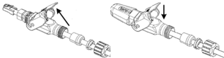
Figure 35: Align RJ45 into Holder
