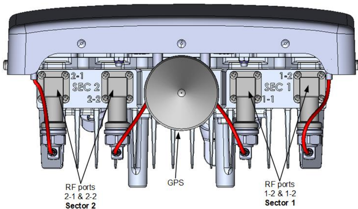
Figure 2: AirSpeed 2900 Top Ports (with integrated antenna)
