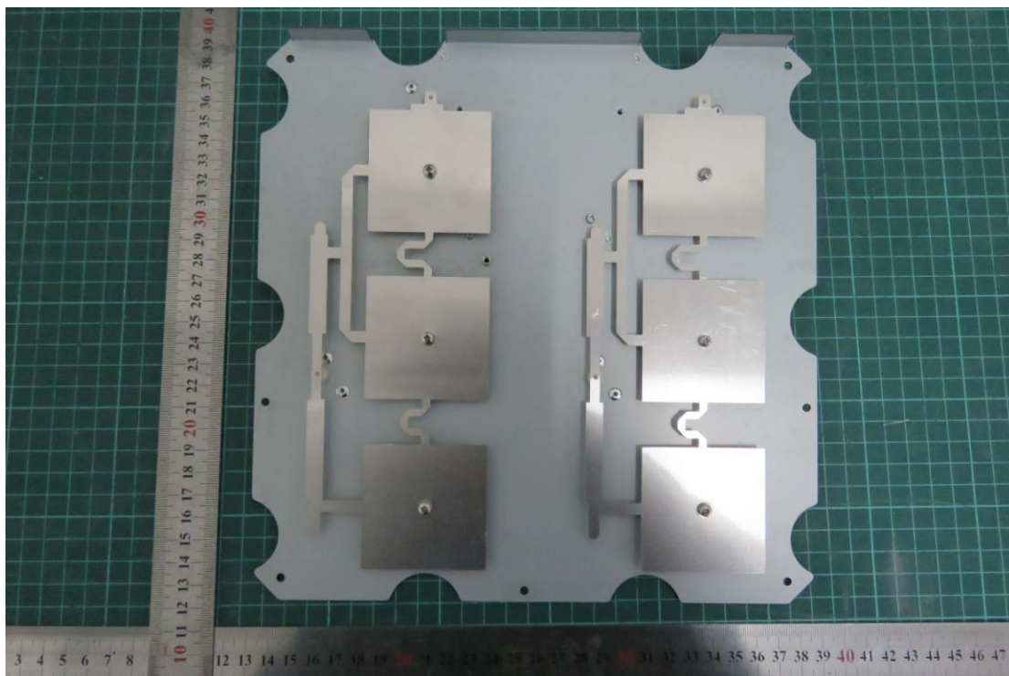
Antenna photo
