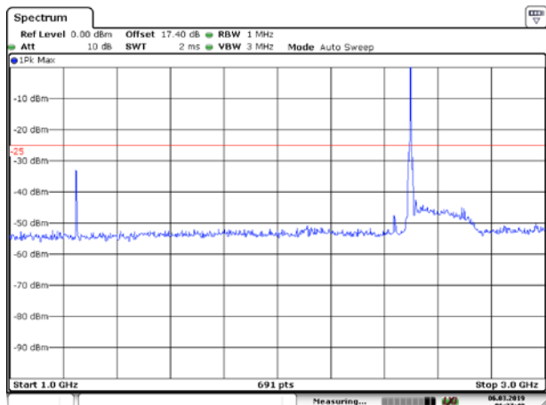
LTE Band 41 5MHz CH-Middle 1GHz~3GHz
