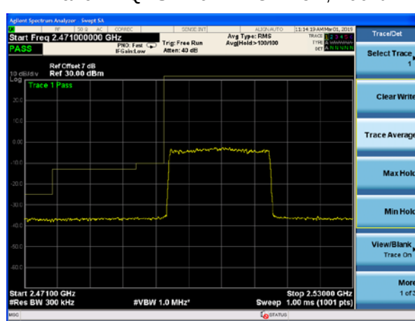
LTE Band 41 QPSK 20MHz CH-Low, 100%RB
