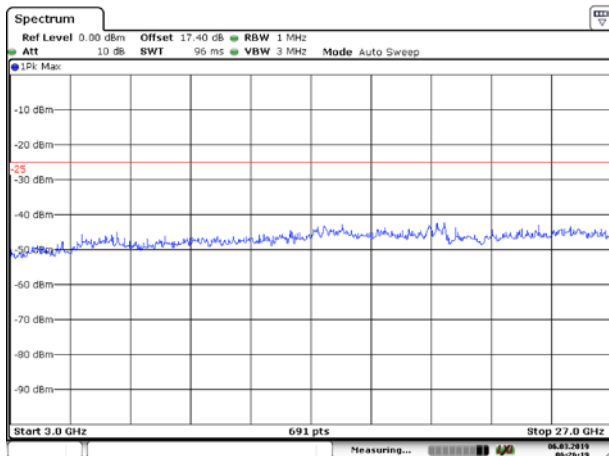
LTE Band 41 5MHz CH-Middle 3GHz~27GHz
