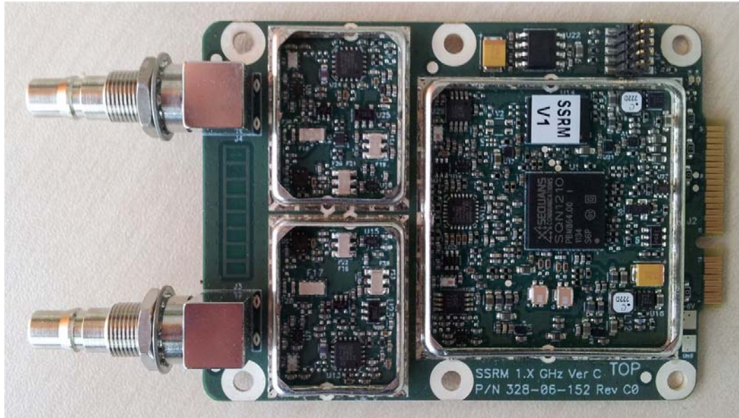
Photograph No.1 SSRM 1.4 GHz module without shielding
