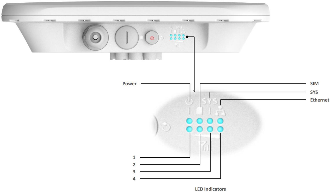
Figure 2: LED panel
