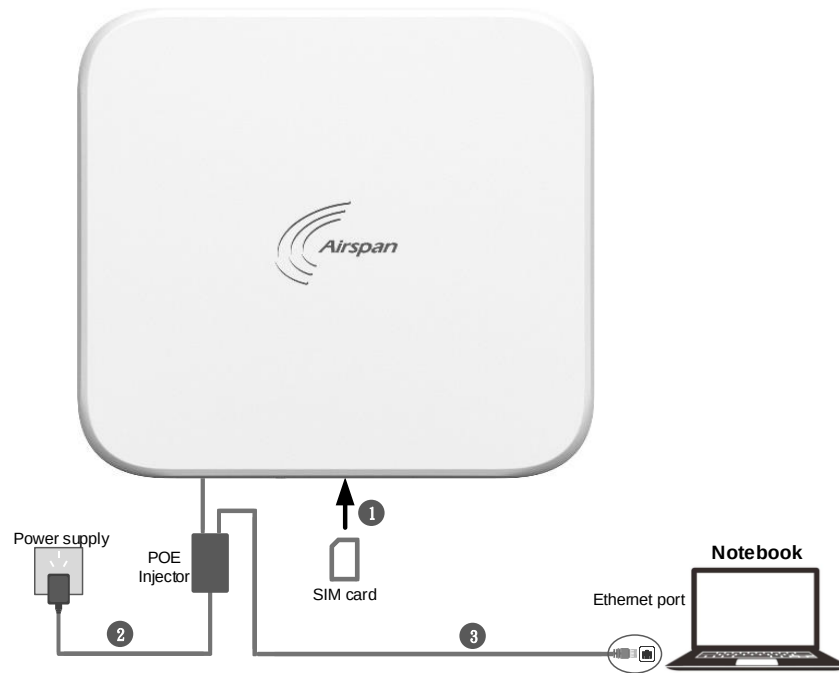
Figure 3: Hardware connection
