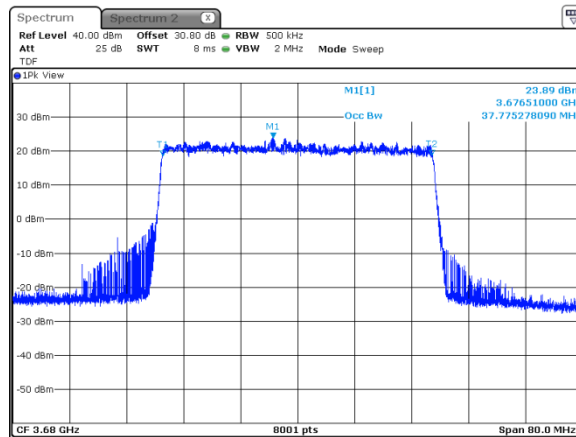
Plot 7.3.48 Occupied bandwidth test result at high frequency
