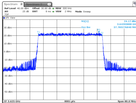
Plot 7.3.42 Occupied bandwidth test result at mid frequency
