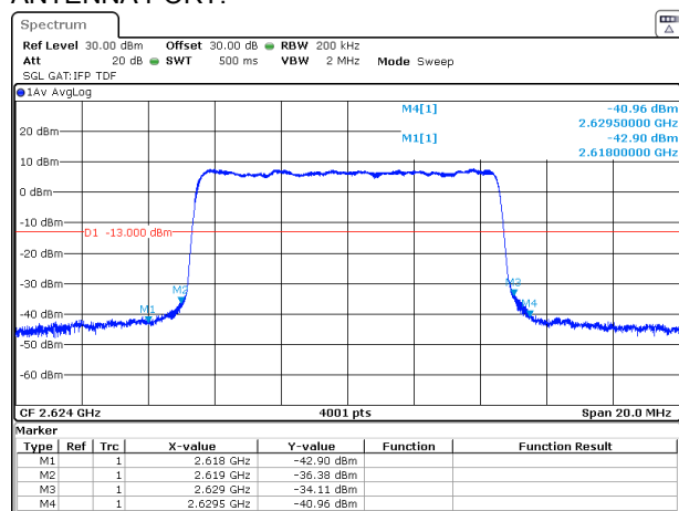
Plot 7.3.24 Spurious emission at band edges test results at high carrier frequency
