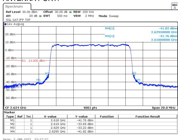
Plot 7.3.27 Spurious emission at band edges test results at high carrier frequency
