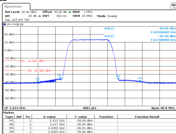
Plot 7.3.24 Spurious emission at band edges test results at high carrier frequency
