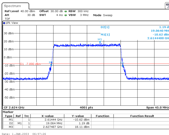
Plot 7.1.18 Occupied bandwidth test result at high frequency, 20 MHz EBW, 64QAM, RF chain #22
