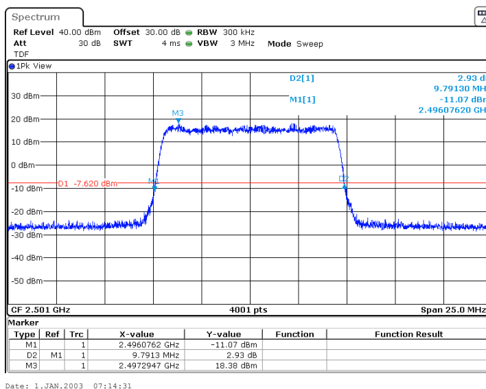
Plot 7.1.26 Occupied bandwidth test result at mid frequency, 10 MHz EBW, 64QAM, RF chain #12
