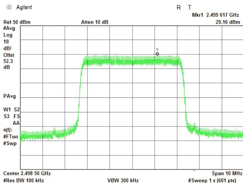
Plot 7.4.1 Power spectral density test results at low frequency, QPSK, 5 MHz EBW, RF # 1
