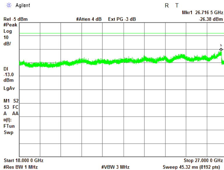
Plot 7.10.25 Spurious emission measurements in 18000-27000 MHz range at low carrier frequency
