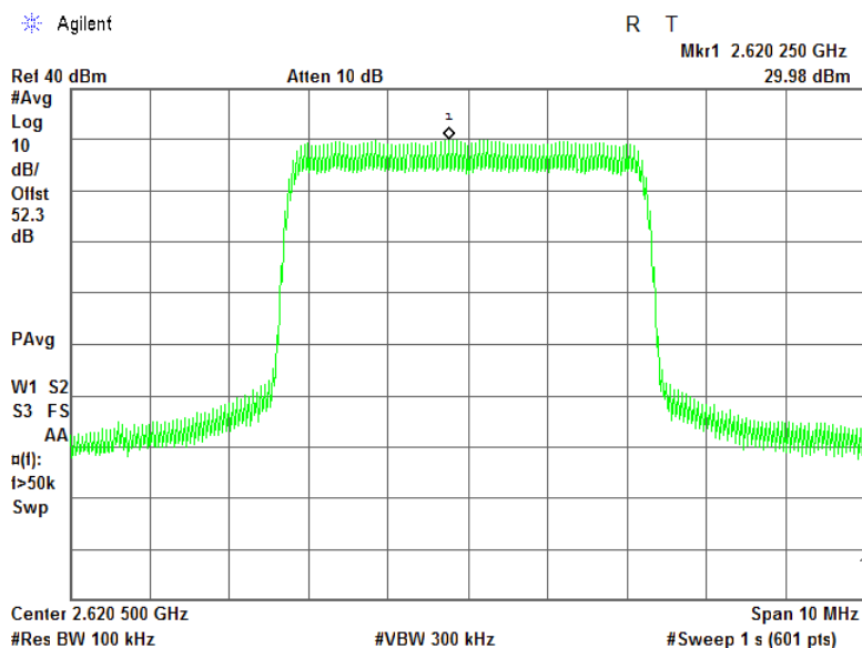
Plot 7.6.19 Power spectral density test results at low frequency, QPSK, 5 MHz EBW, RF # 2
