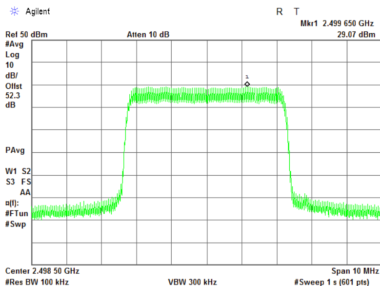
Plot 7.5.1 Power spectral density test results at low frequency, QPSK, 5 MHz EBW, RF # 1
