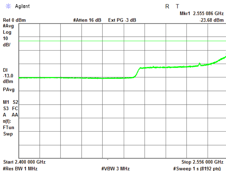
Plot 7.11.15 Spurious emission measurements in 2400 - 2556 MHz at high carrier frequency
