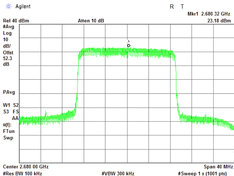
Plot 7.6.33 Power spectral density test results at high frequency, QPSK, 20 MHz EBW, RF # 2
