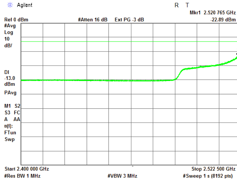
Plot 7.11.13 Spurious emission measurements in 2400 – 2522.5 MHz at mid carrier frequency
