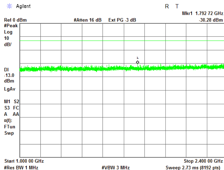
Plot 7.11.14 Spurious emission measurements in 1000 - 2400 MHz at high carrier frequency
