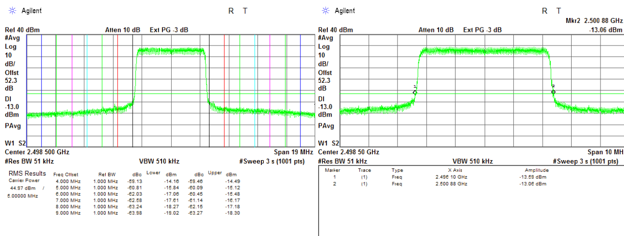
Plot 7.8.2 Spurious emission at band edges test results at mid carrier frequency, 5 MHz EBW
