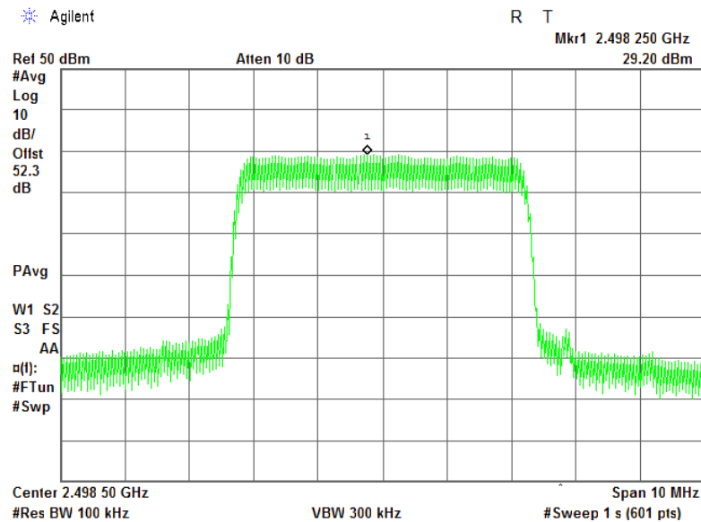
Plot 7.5.19 Power spectral density test results at low frequency, QPSK, 5 MHz EBW, RF # 2
