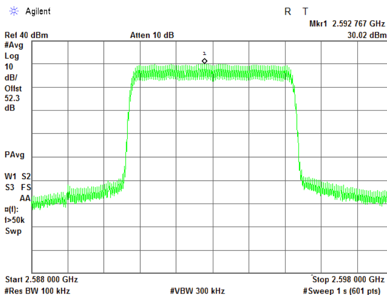
Plot 7.4.23 Power spectral density test results at mid frequency, 64QAM, 5 MHz EBW, RF # 2
