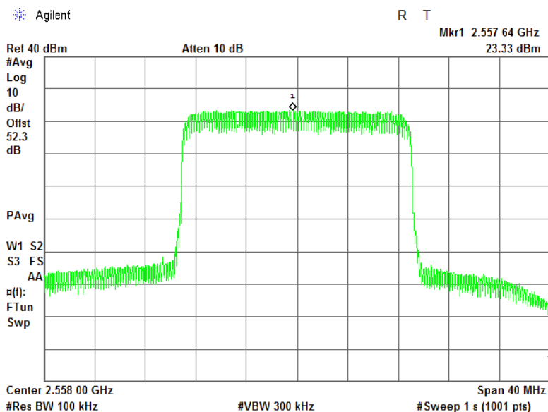
Plot 7.5.33 Power spectral density test results at high frequency, QPSK, 20 MHz EBW, RF # 2
