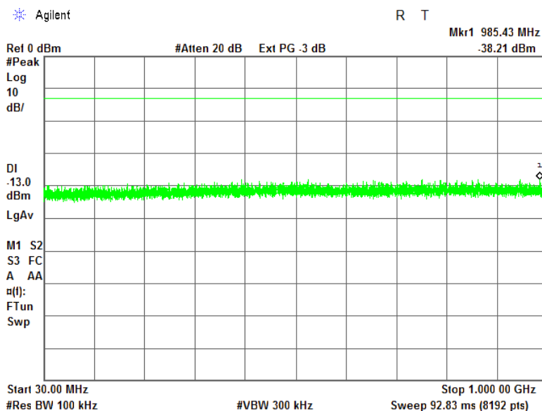
Plot 7.11.7 Spurious emission measurements in 30 - 1000 MHz range at low carrier frequency
