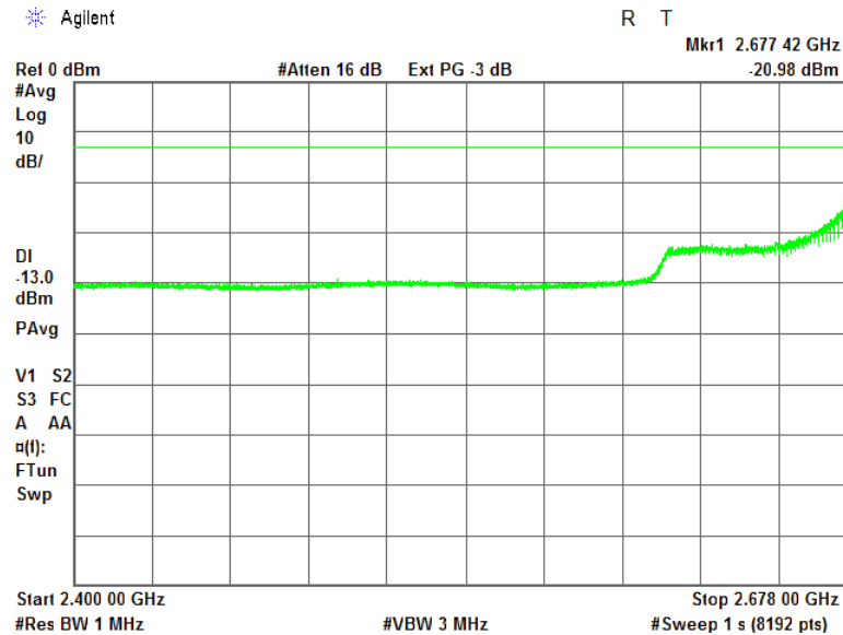
Plot 7.12.15 Spurious emission measurements in 2400 -2678 MHz at high carrier
