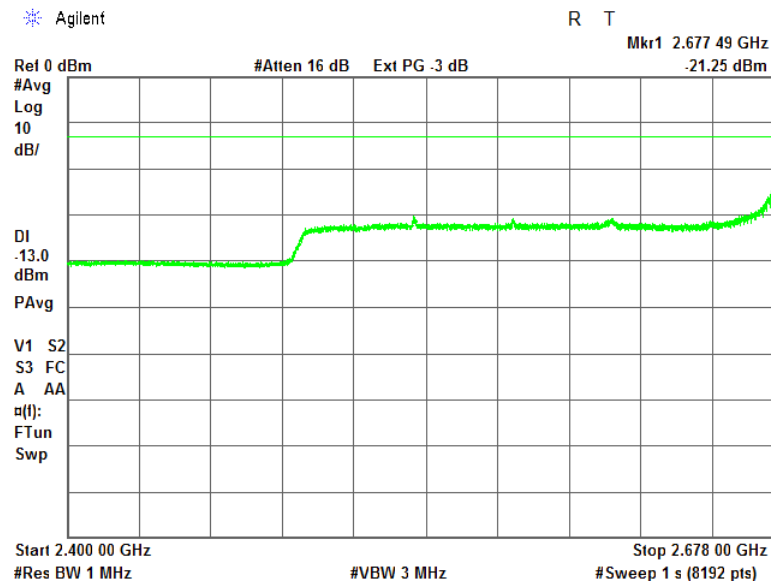
Plot 7.10.15 Spurious emission measurements in 2400 -2678 MHz at high carrier
