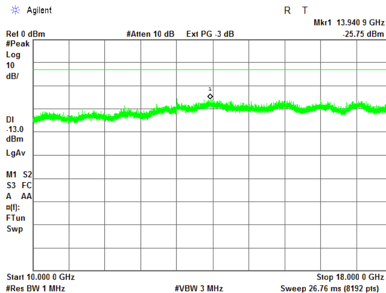
Plot 7.12.22 Spurious emission measurements in 10000-18000 MHz range at low carrier frequency
