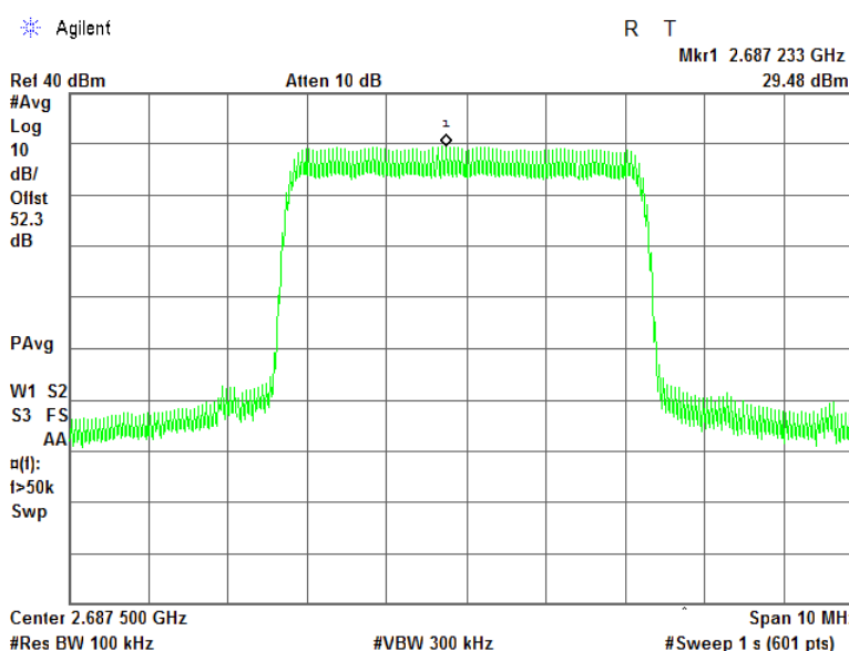
Plot 7.4.24 Power spectral density test results at high frequency, 64QAM, 5 MHz EBW, RF # 2
