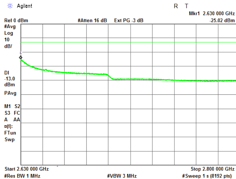
Plot 7.12.16 Spurious emission measurements in 2630 - 2800 MHz range at low carrier frequency
