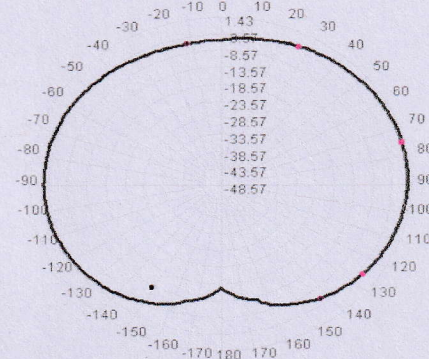
Total(H-XY), Max= 0.24dBi, CirD=18.06
