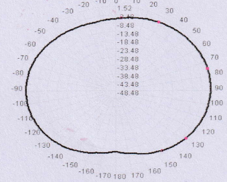
Total(H-XY), Max= 0.64dBi, CirD=12.97
