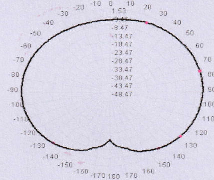
Total(H-XY), Max= 0.22dBi, CirD=20.07
