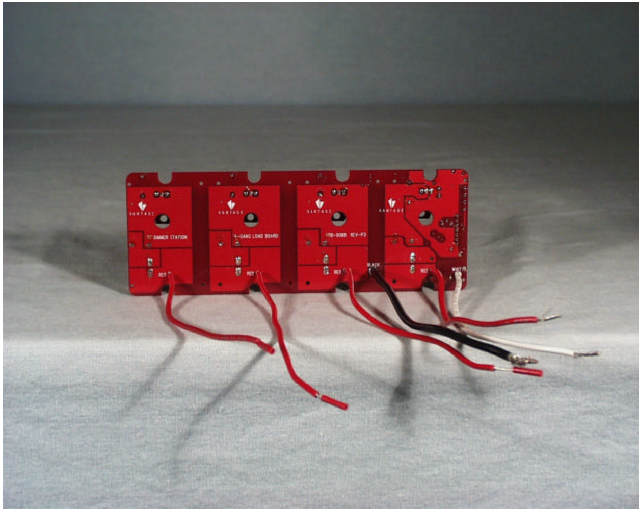
Back View Of The RDS4-2A Load PCB
