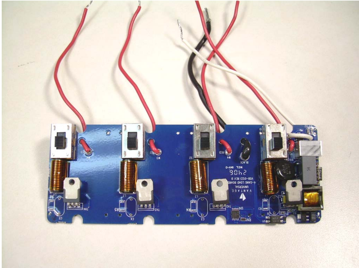
Photograph 9 - Front Side of the Dimmer PCB
