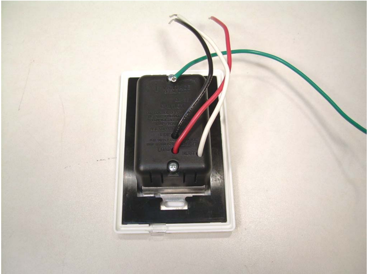
Photograph 15 - Back View of the Rx single gang
