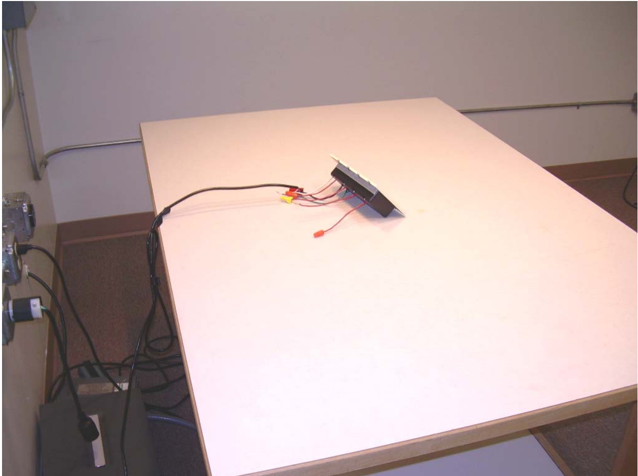
Photograph 4 - Back View Conducted Disturbance Worst Case Configuration
