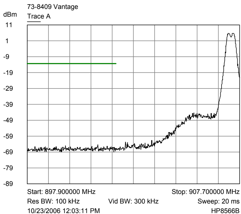
Trace A Lower channel band edge plot - 100 kHz RBW and 10 MHz span
