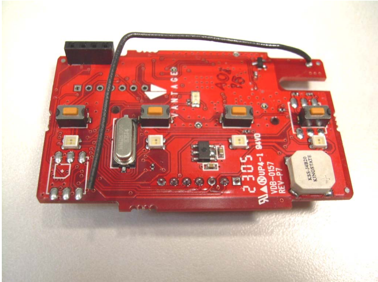
Photograph 20 - Front Side of the Switch/Transceiver PCB
