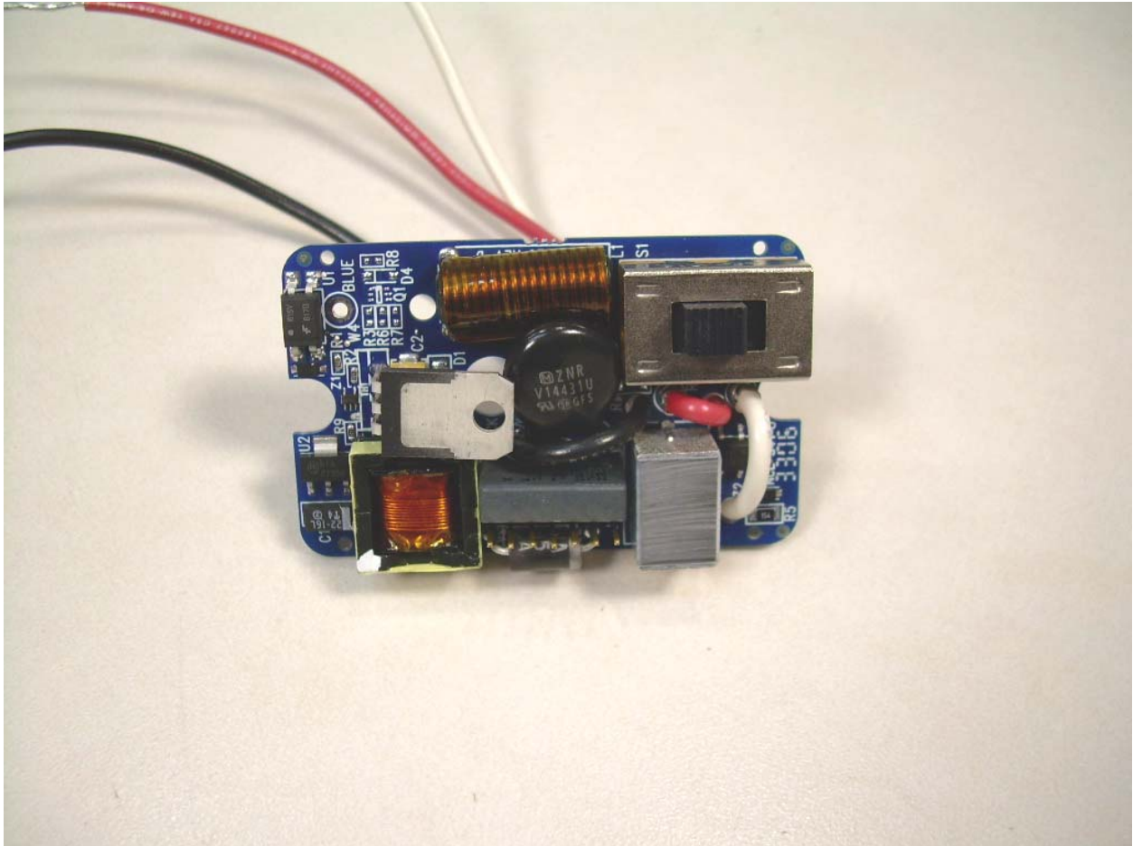
Photograph 18 - View of the Component Side of the Dimmer PCB
