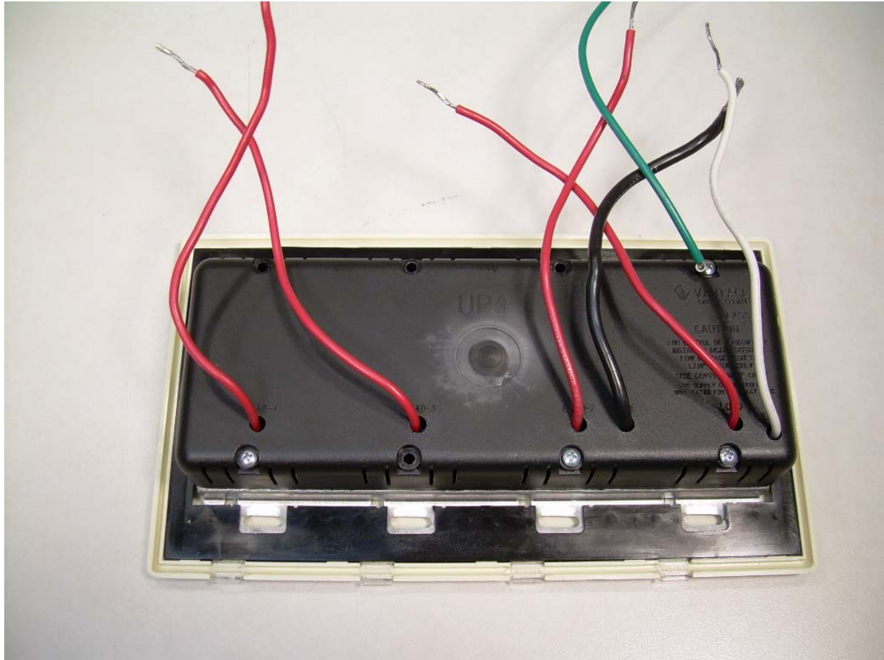
Photograph 6 - Back View of the Rx 4 gang
