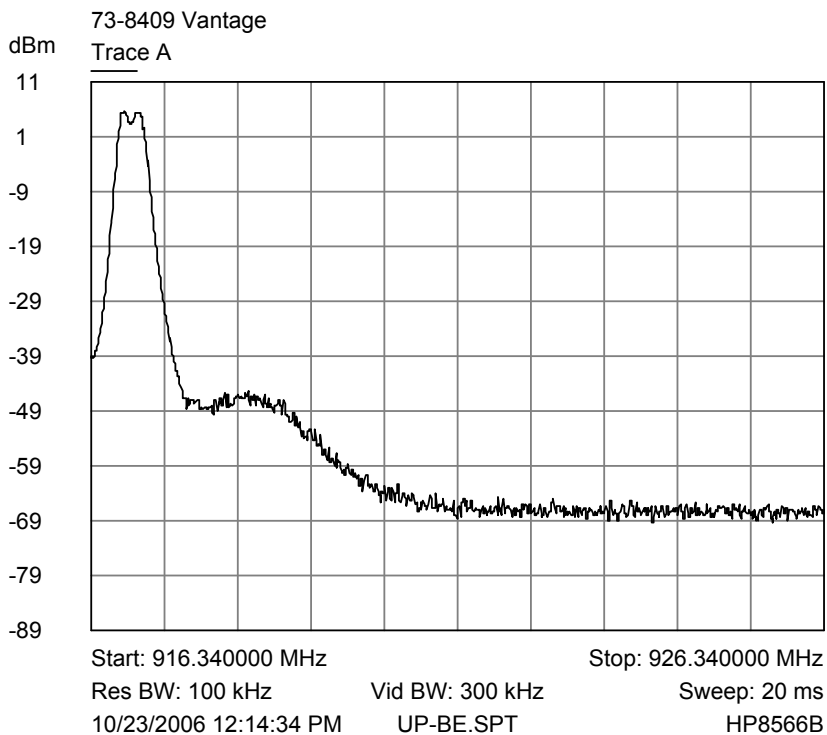
Trace A Upper channel band edge plot - 100 kHz RBW and 10 MHz span
