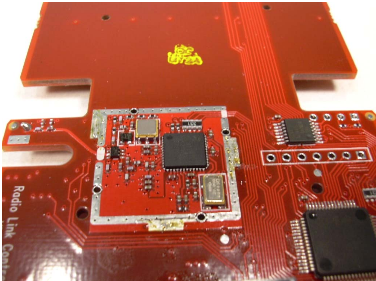
Photograph 13 - View of the Transceiver Circuit
