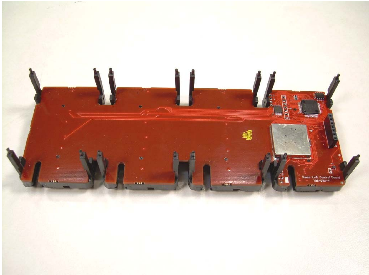
Photograph 12 - Back Side of the Switch/Transceiver PCB
