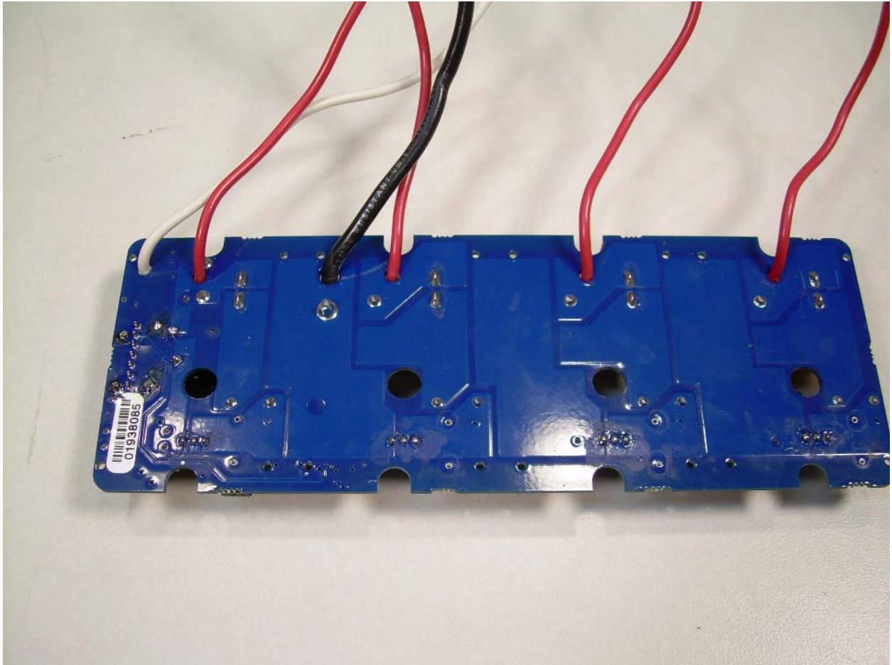
Photograph 10 - Back Side of the Dimmer PCB
