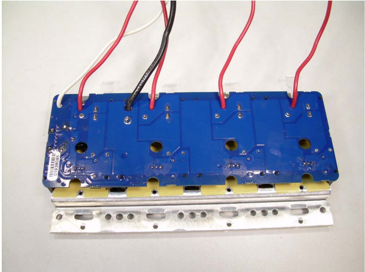
Photograph 8 - Rear Cover Removed
