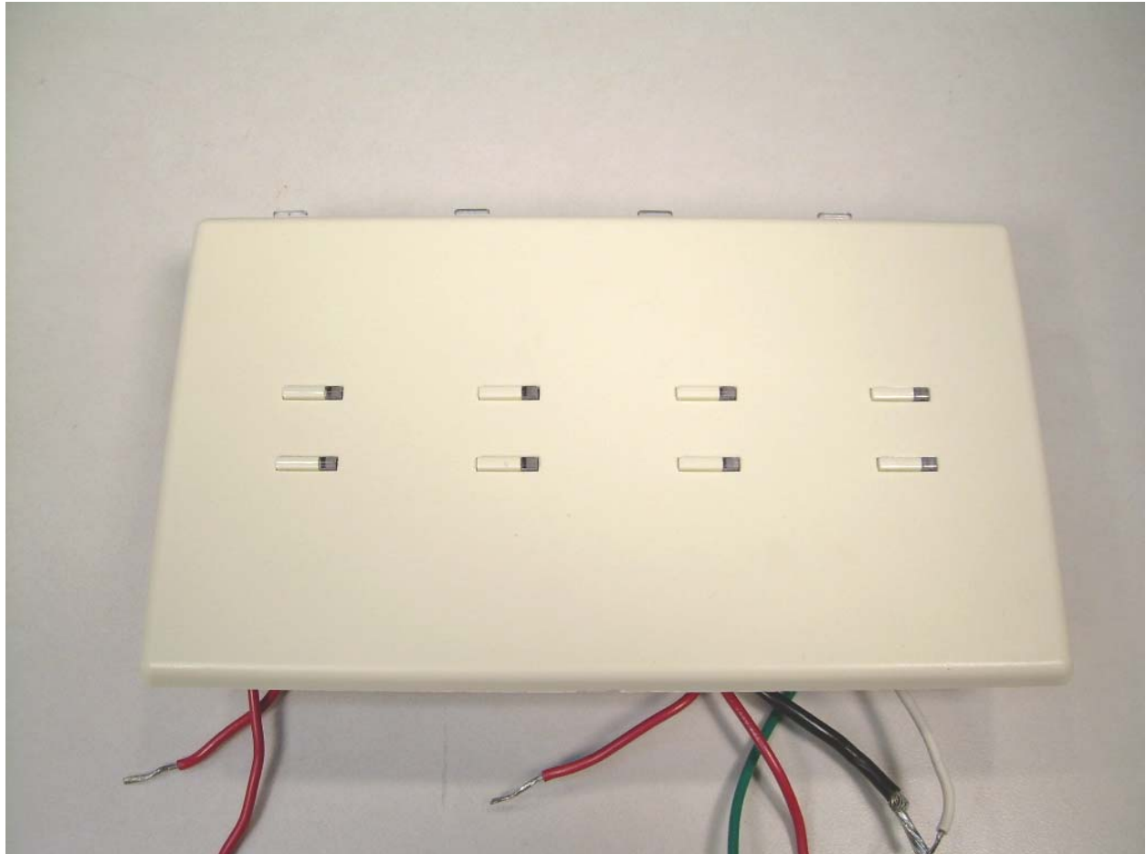
Photograph 5 - Front View of the Rx 4 gang
