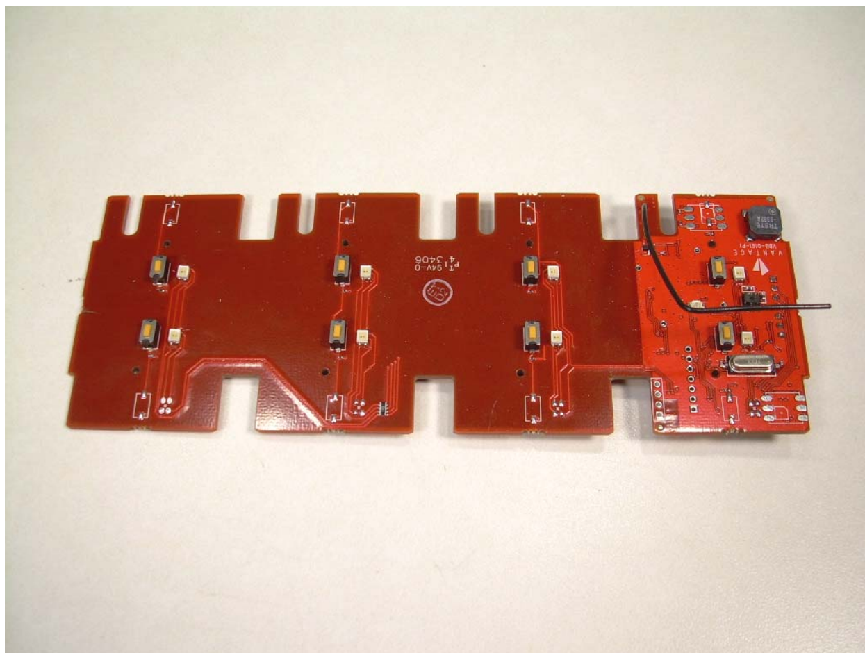
Photograph 11 - Front Side of the Switch/Transceiver PCB
