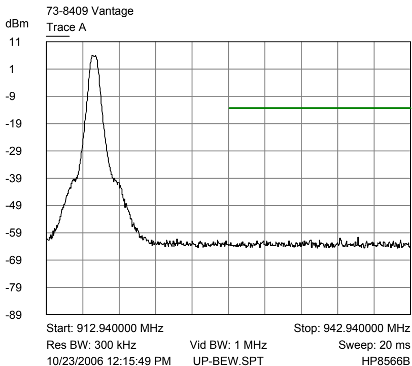
Trace A Upper channel band edge plot - 300 kHz RBW and 30 MHz span
