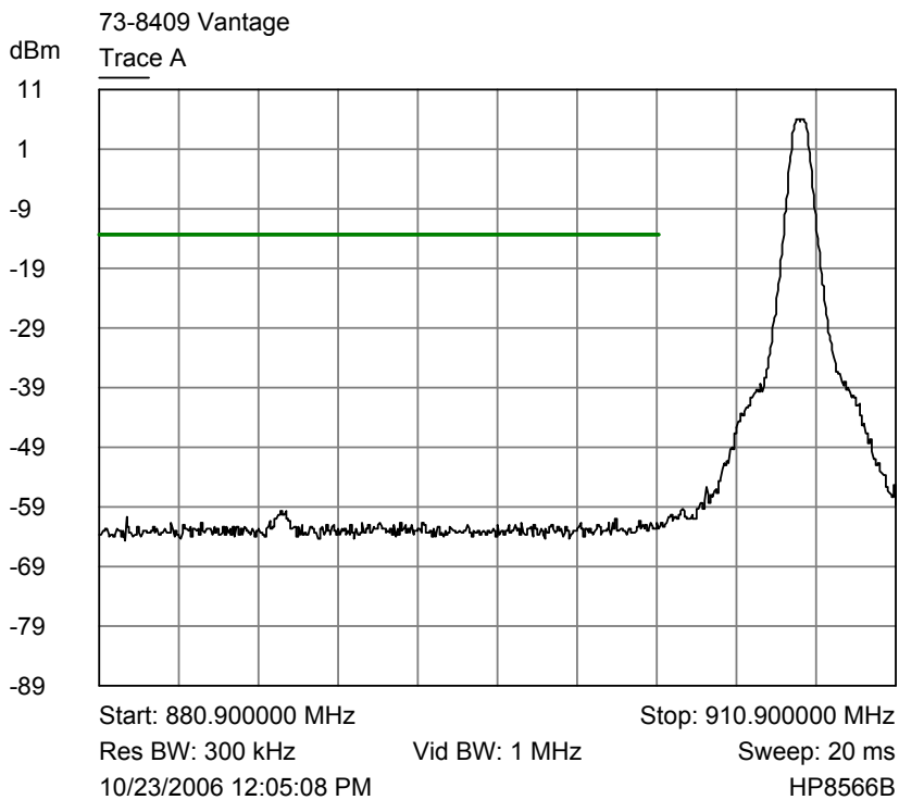
Trace A Lower channel band edge plot - 300 kHz RBW and 30 MHz Span
