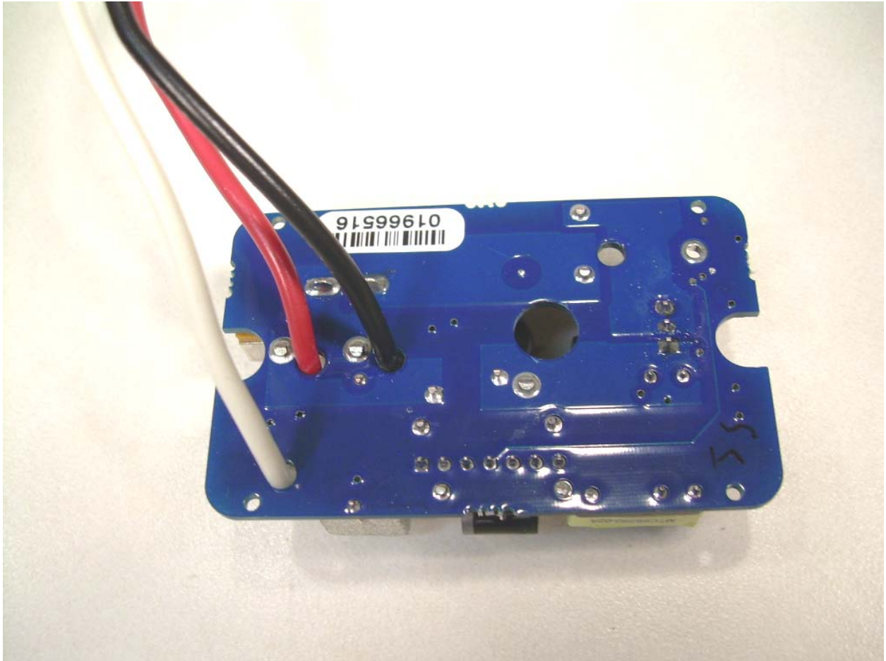
Photograph 19 - View of the Trace Side of the Dimmer PCB
