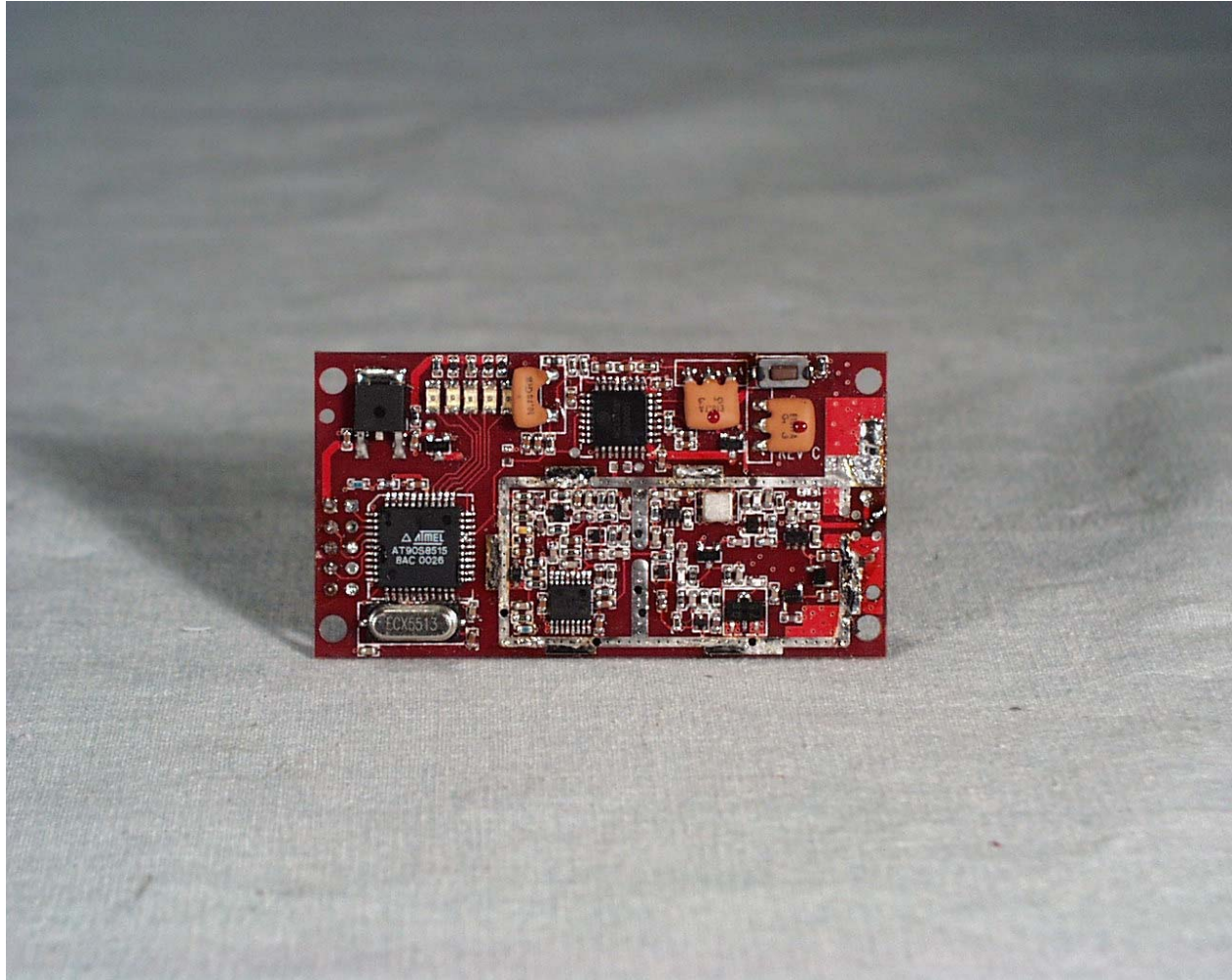
Top View of the RF Daughter Board with Shield Removed
