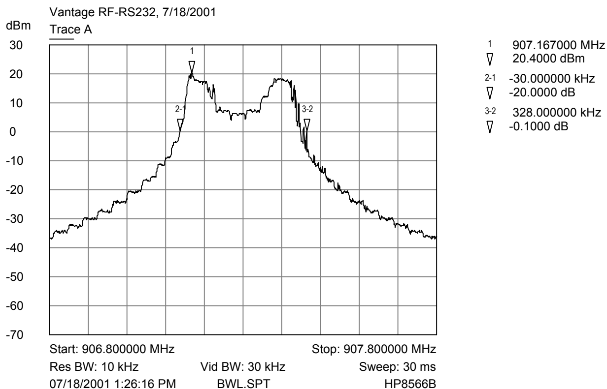
Emission Bandwidth Plot - (Low Channel)
