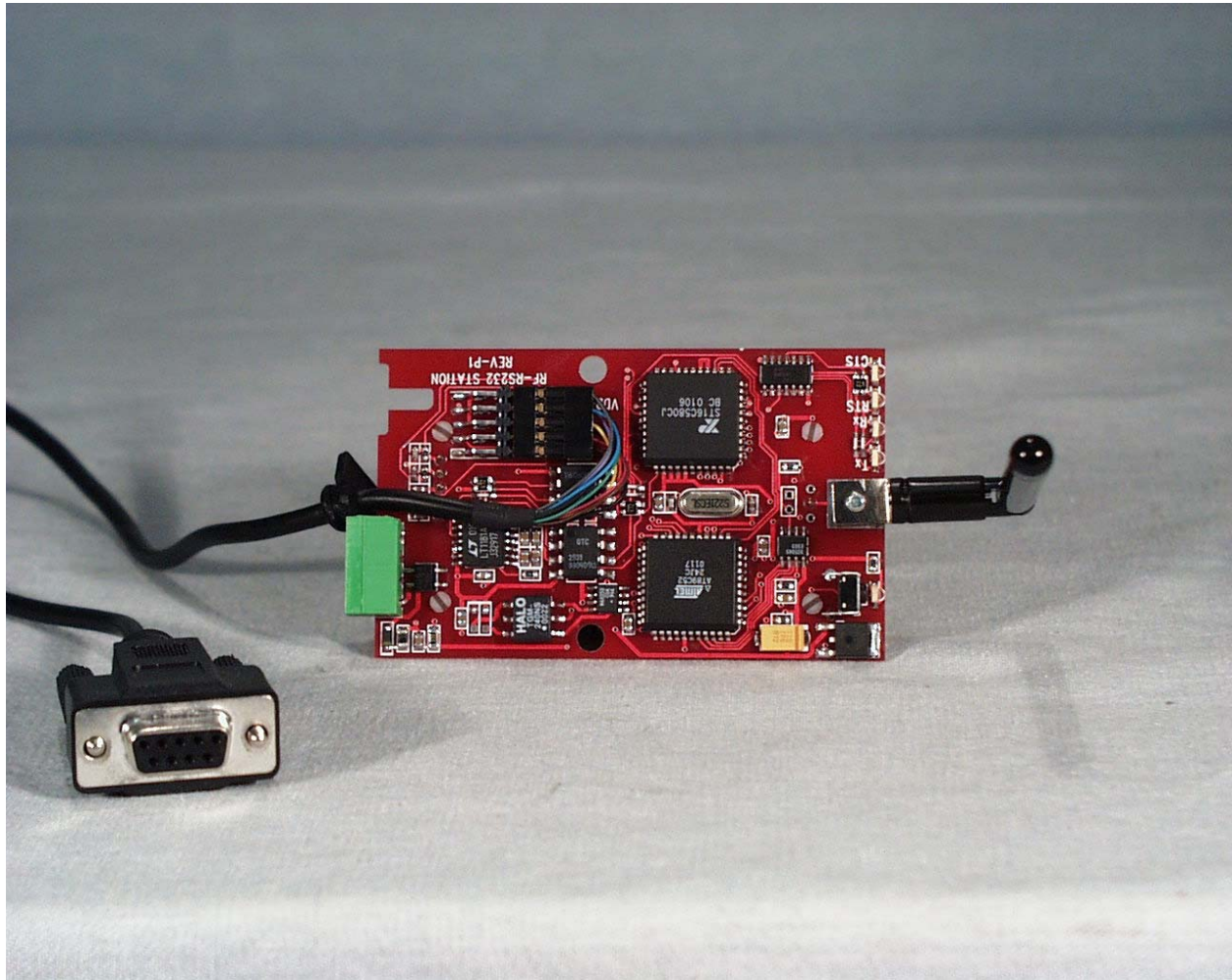
Top View of the S232RF PCB
