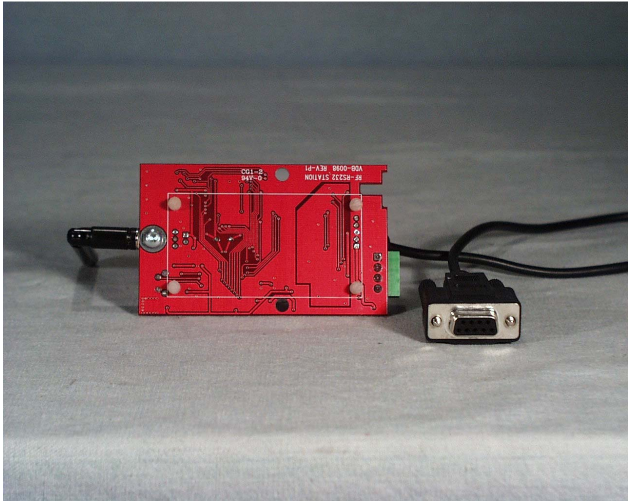
Bottom View of the S232RF PCB without RF Daughter Board
