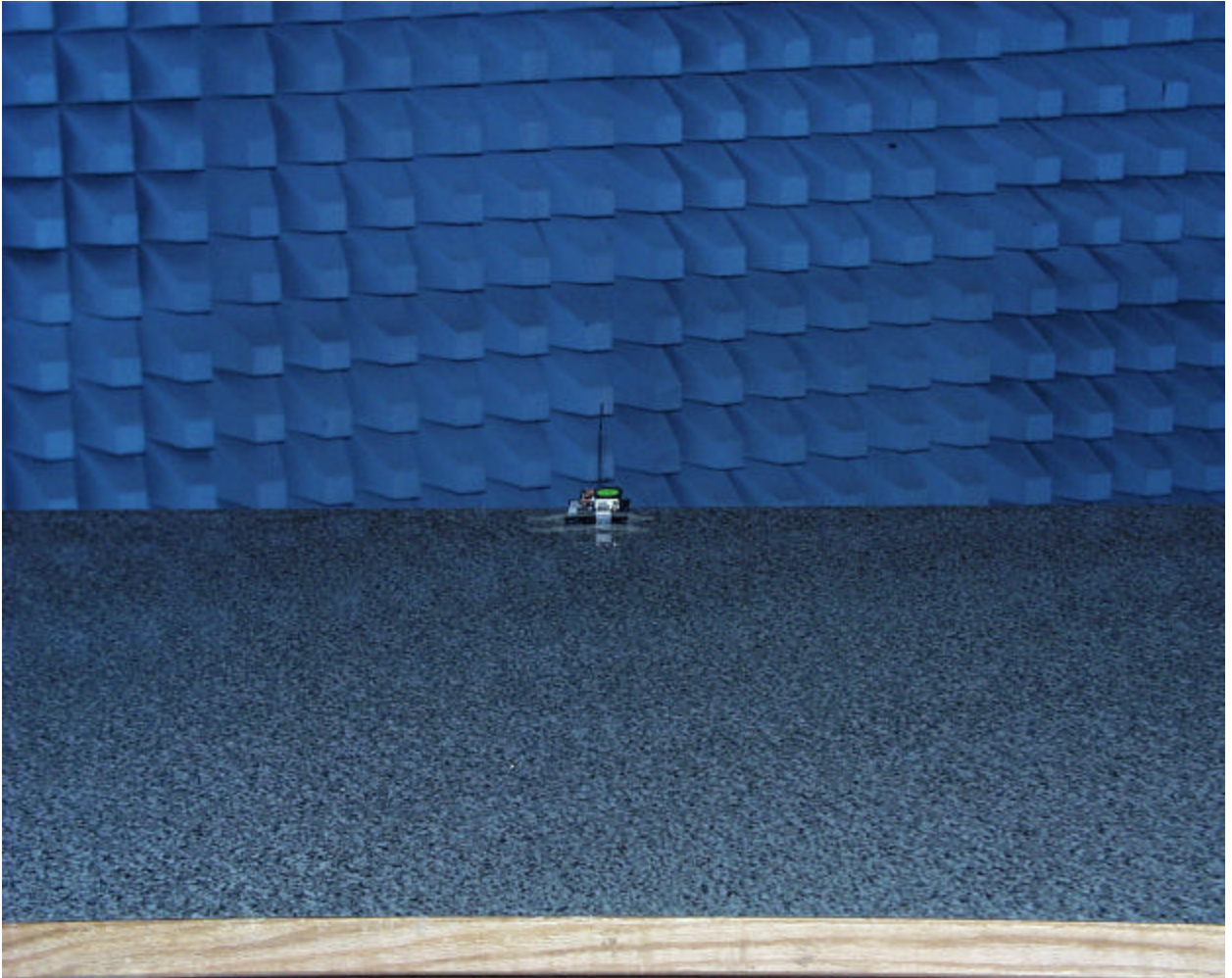
Back View Of Radiated Test Setup
