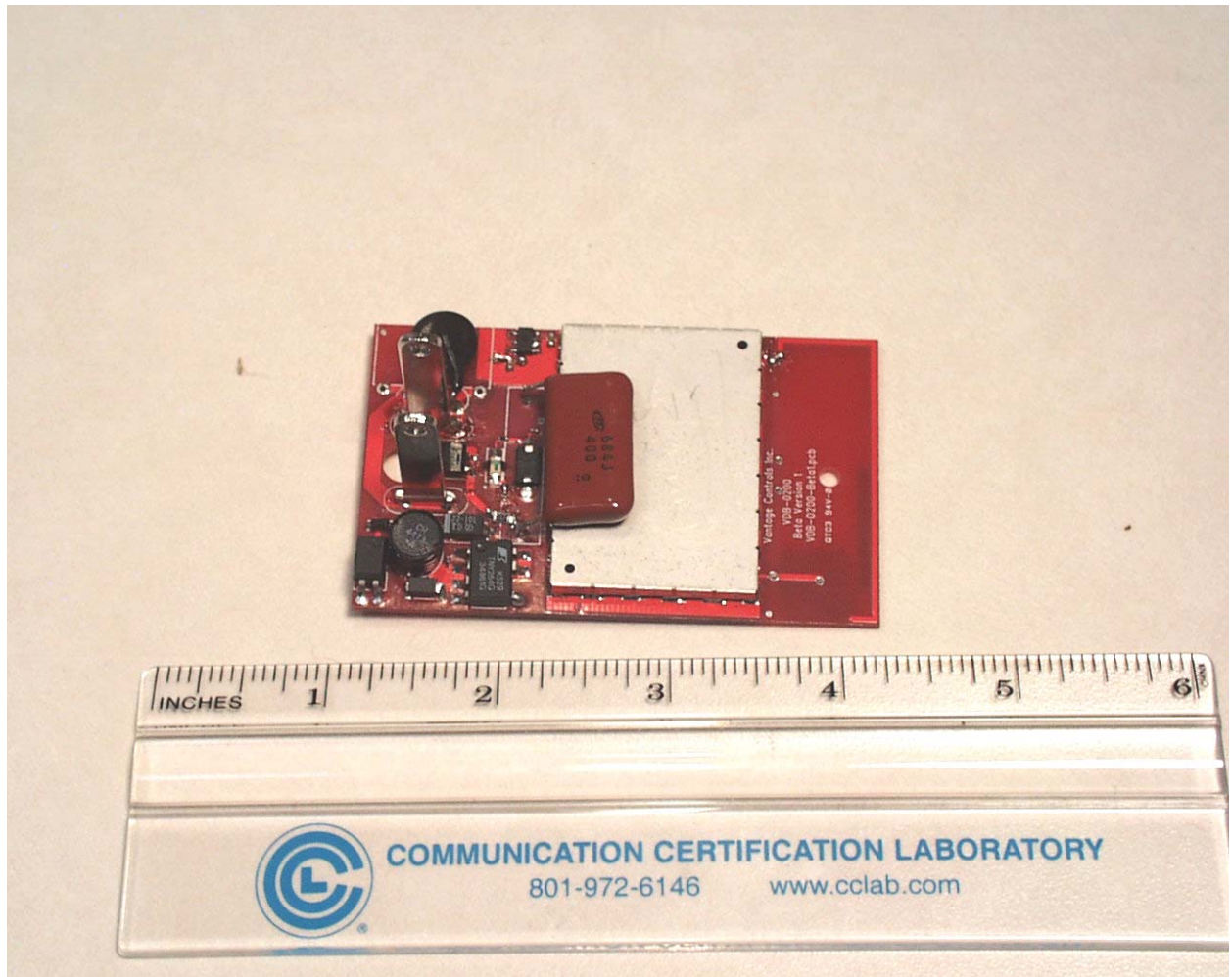
Component Side of the PCB with Shield in Place
