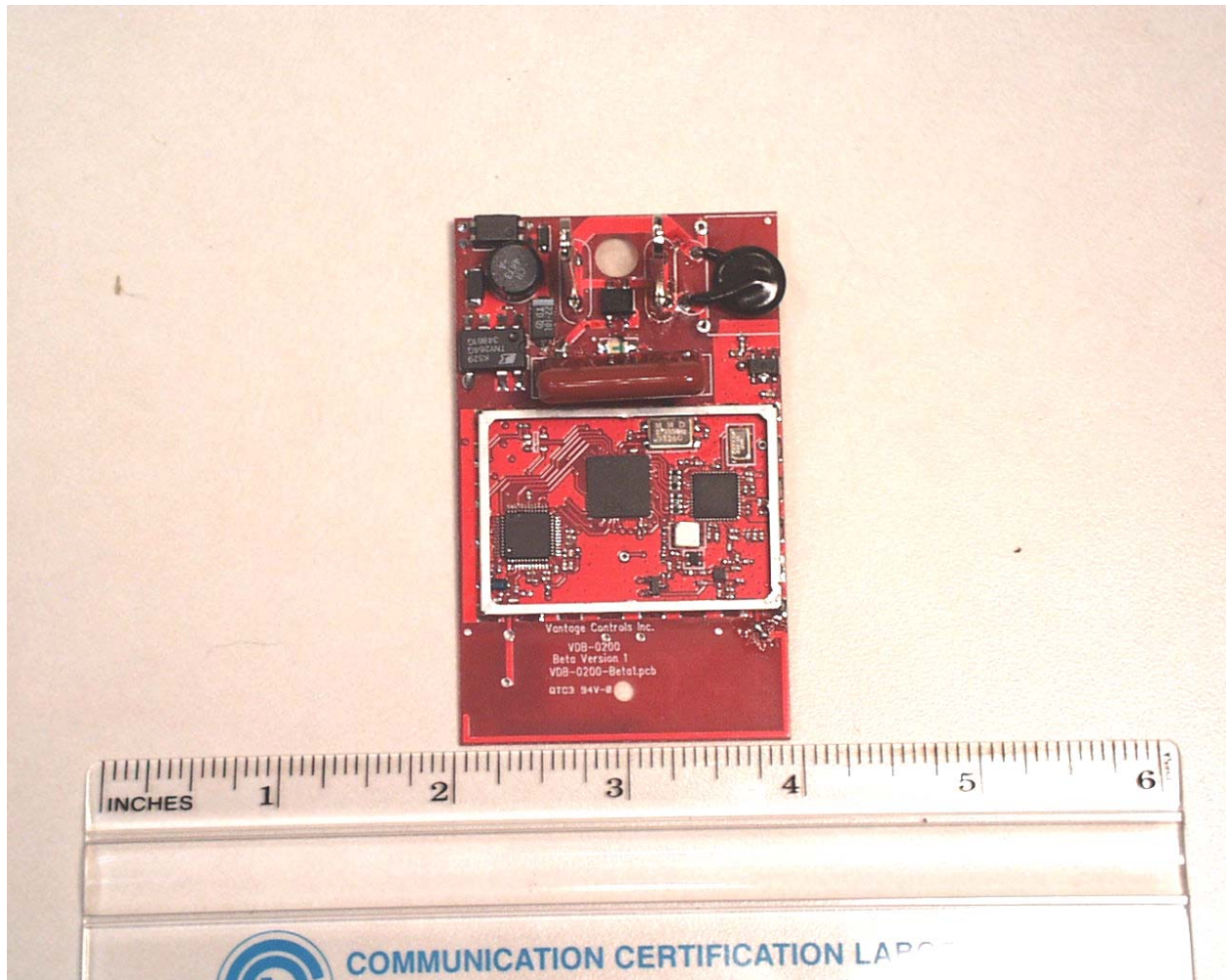
Component Side of the PCB with Shield Removed
