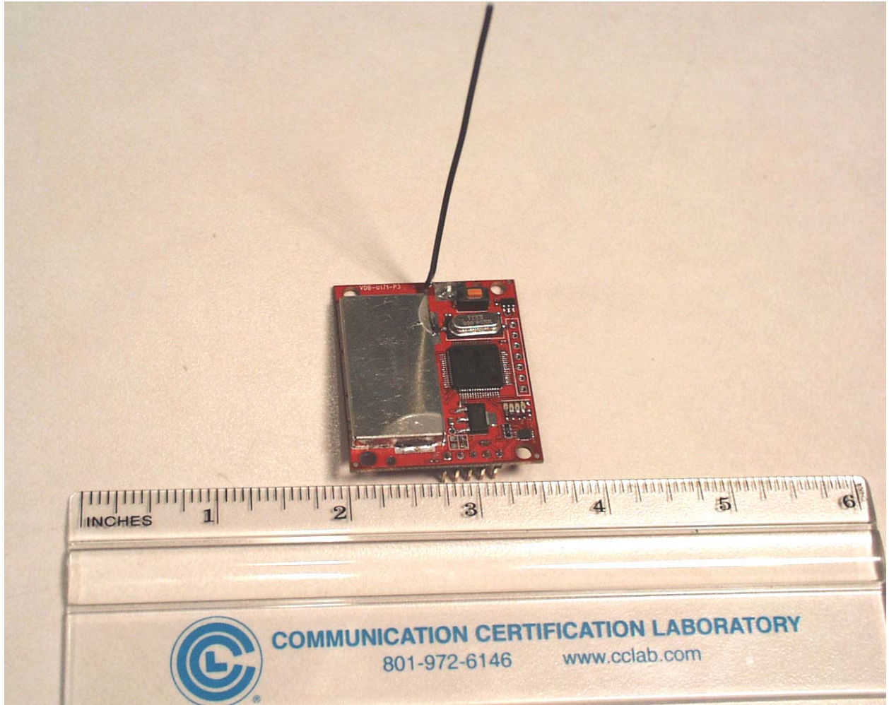
Top View of the EUT With RF Shielding in Place
