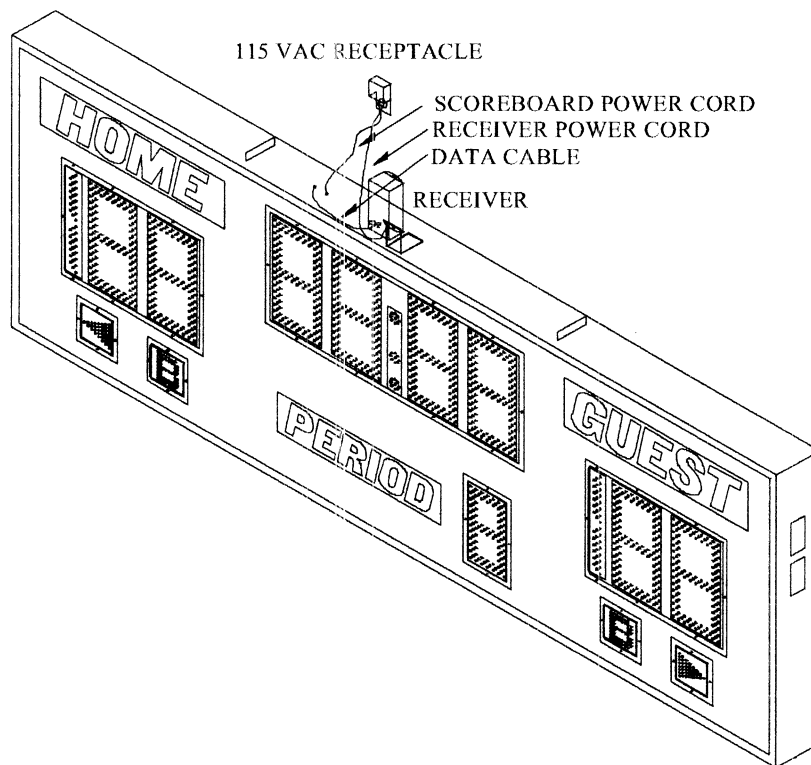
Figure 3 SCORELINK 200 Receiver Installation
