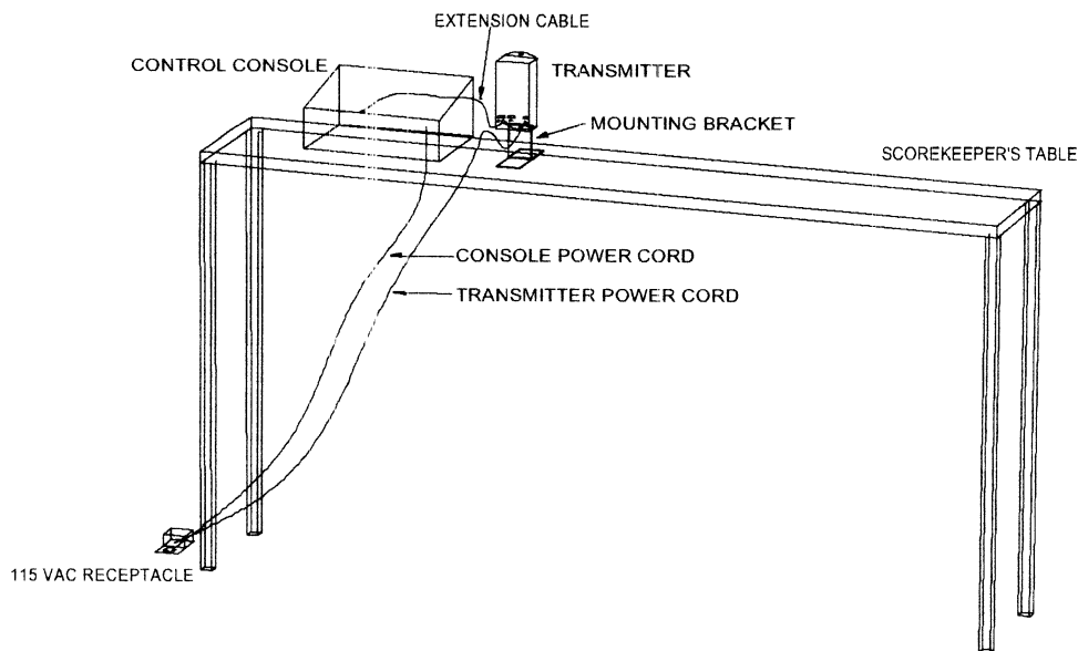
Figure 1 SCORELINK 200 Transmitter Installation
