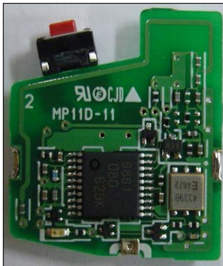
PCB Top View
