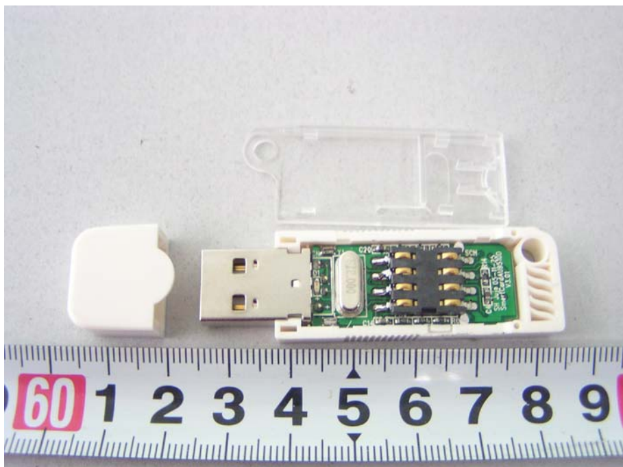
EUT-Inside View (2)
