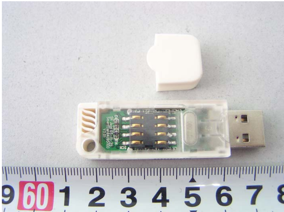
EUT-Inside View (1)
