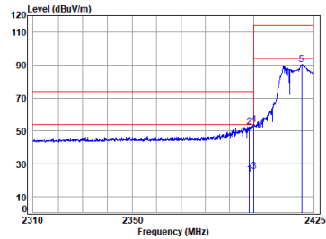
car 2.4G SRD_TX_CH_L_Vertical
