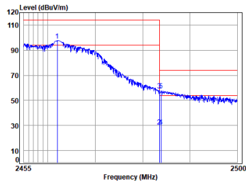
car 2.4G SRD_TX_CH_H_Horizontal
