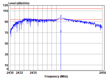
car 2.4G SRD_TX_CH_M_Horizontal
