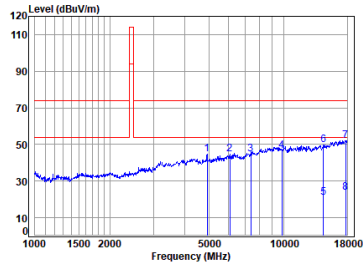
car 2.4G SRD_TX_CH_H_Horizontal
