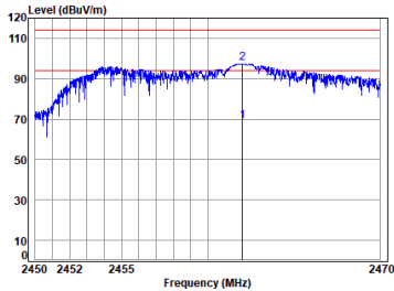
car 2.4G SRD_TX_CH_H_Horizontal
