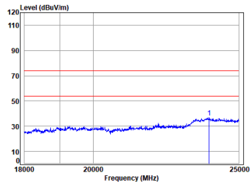
car 2.4G SRD_TX_CH_M_Horizontal
