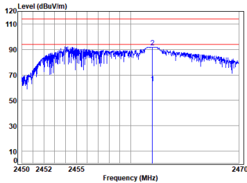
car 2.4G SRD_TX_CH_H_Vertical
