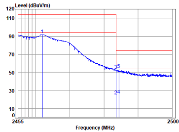
car 2.4G SRD_TX_CH_H_Vertical
