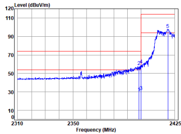
car 2.4G SRD_TX_CH_L_Horizontal
