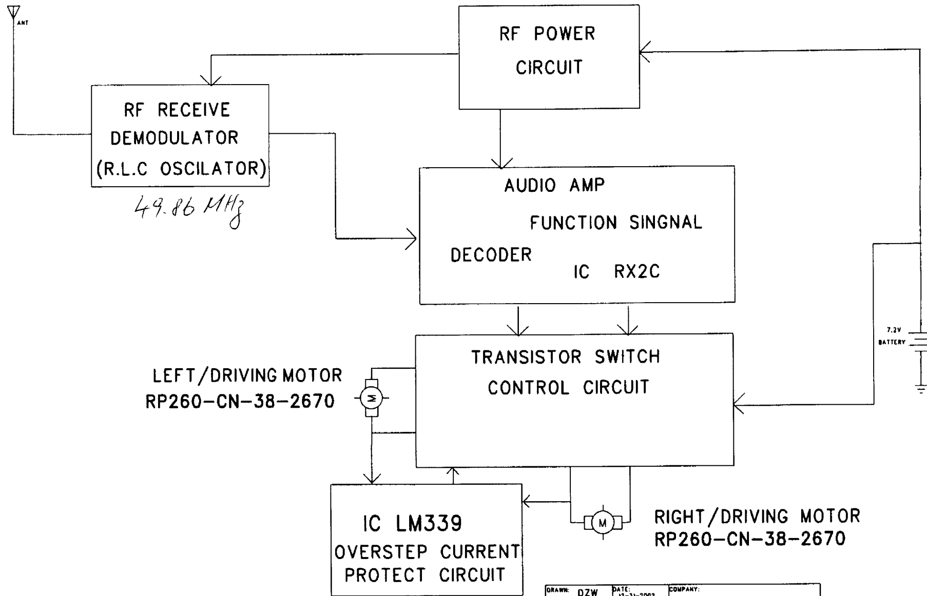
RE WINDER BLOCK DIAGRAM
