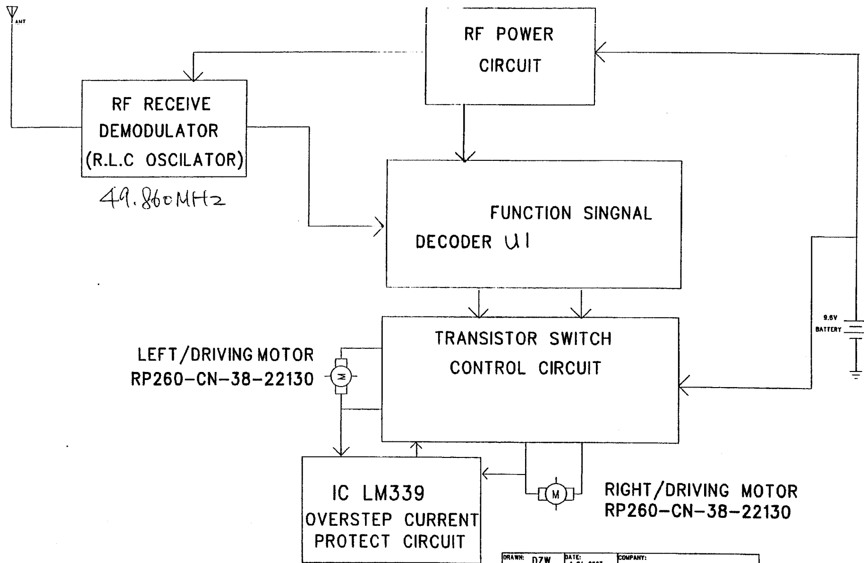
RE WINDER BLOCK DIAGRAM
