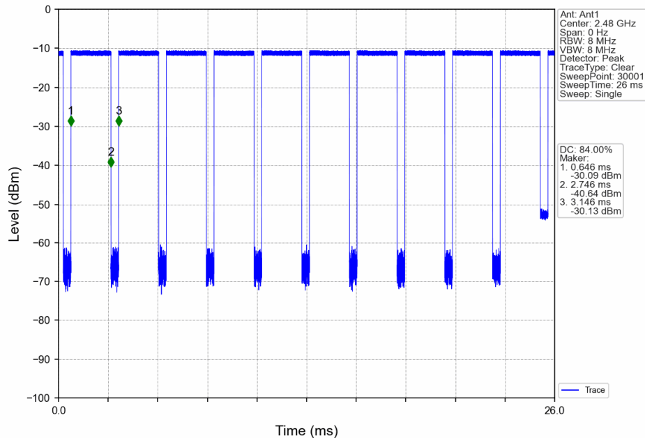
1M_HCH_2480MHz_Ant1_NTNV
