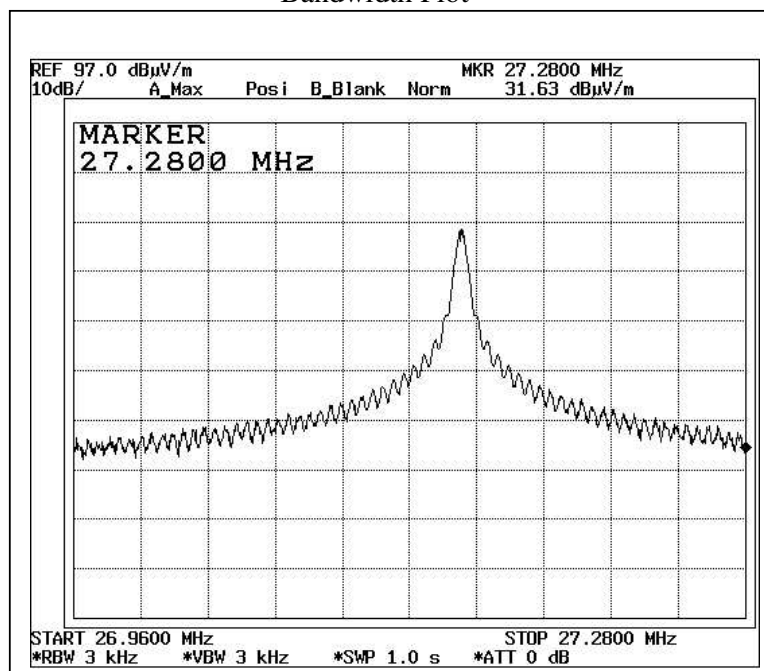
Bandwidth Plot
