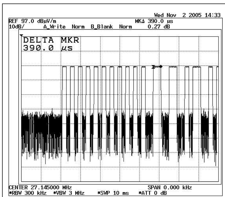
Duty Cycle 3
